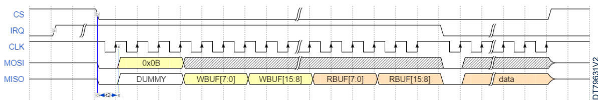
Figure 5. SPI read transaction
