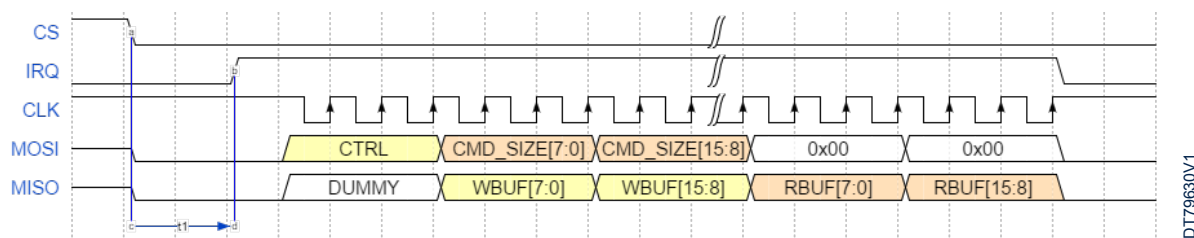
Figure 4. SPI header format
