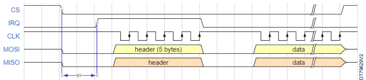
Figure 3. Generic SPI transaction
