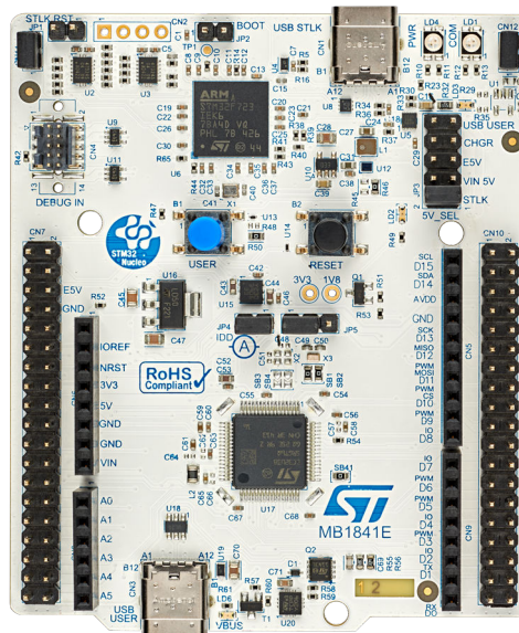
Figure 9. STM32 Nucleo development board (NUCLEO-U385RG-Q)
