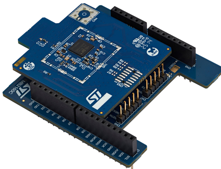
Figure 10. ARDUINO® interface board of X-NUCLEO-WBA25A1 with MCU RF board (STM32WBA55CG or STM32WBA65RI) plugged on top
