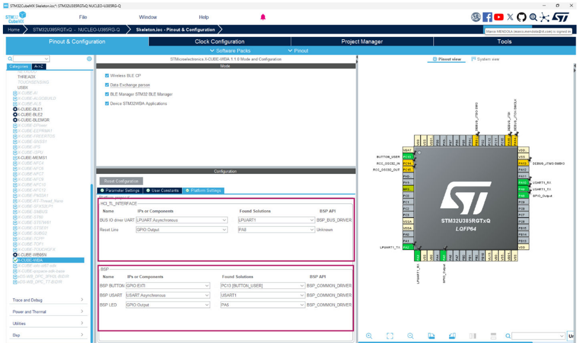
Figure 19. STM32CubeMX - Platform settings
