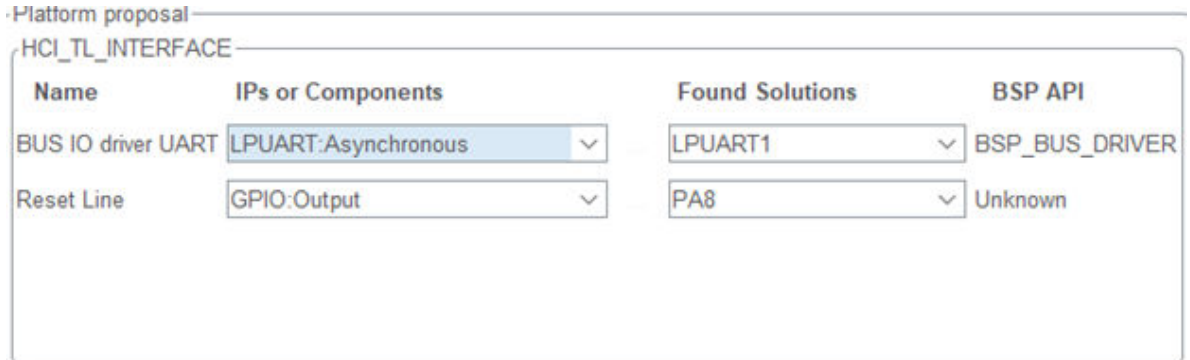
Figure 20. STM32CubeMX - UART protocol configuration
