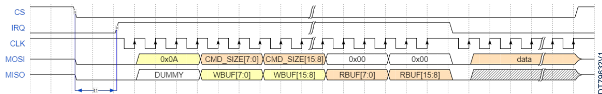
Figure 6. SPI write transaction
