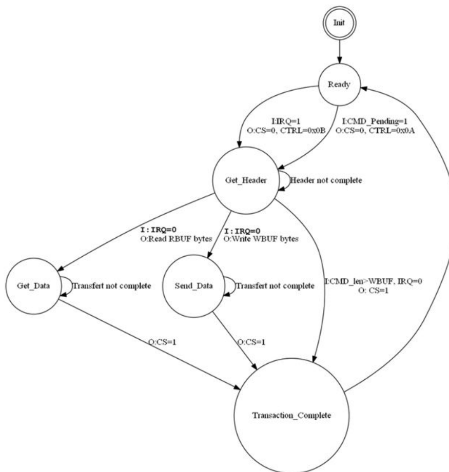
Figure 8. Expected SPI protocol state machine on external microcontroller
