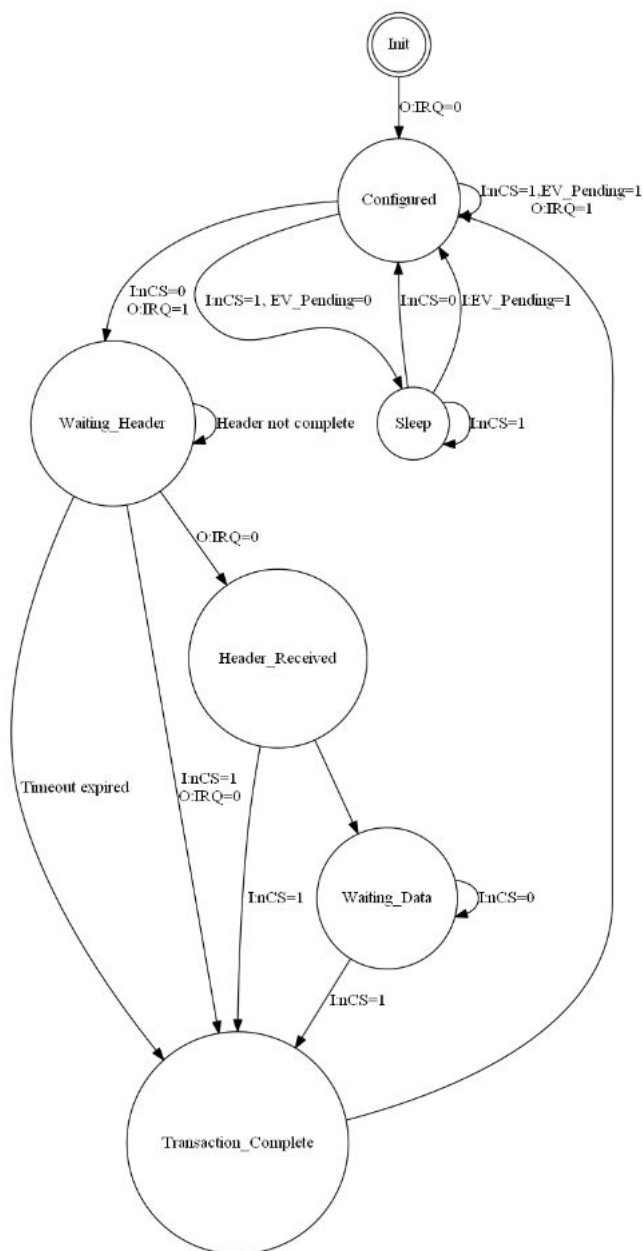
Figure 7. SPI protocol state machine
