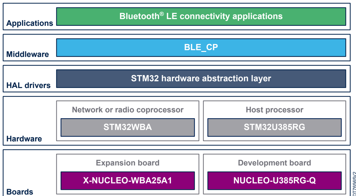
Figure 1. X-CUBE-WBA software architecture
