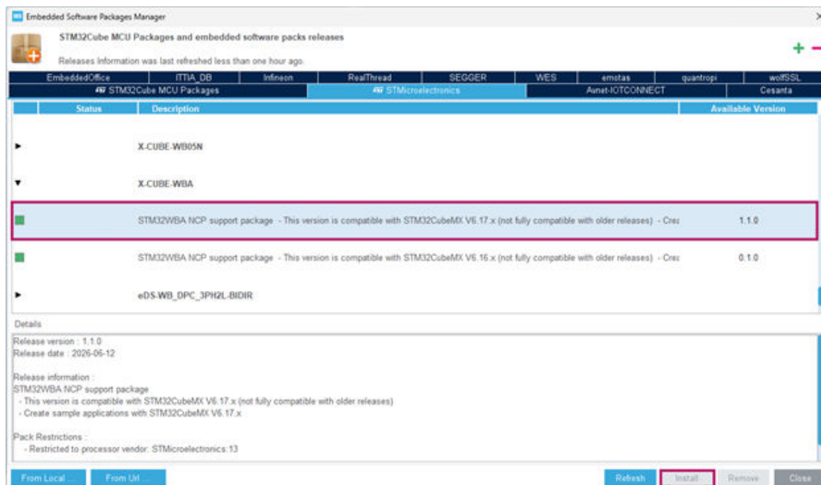
Figure 12. STM32CubeMX - X-CUBE-WBA software package selection
