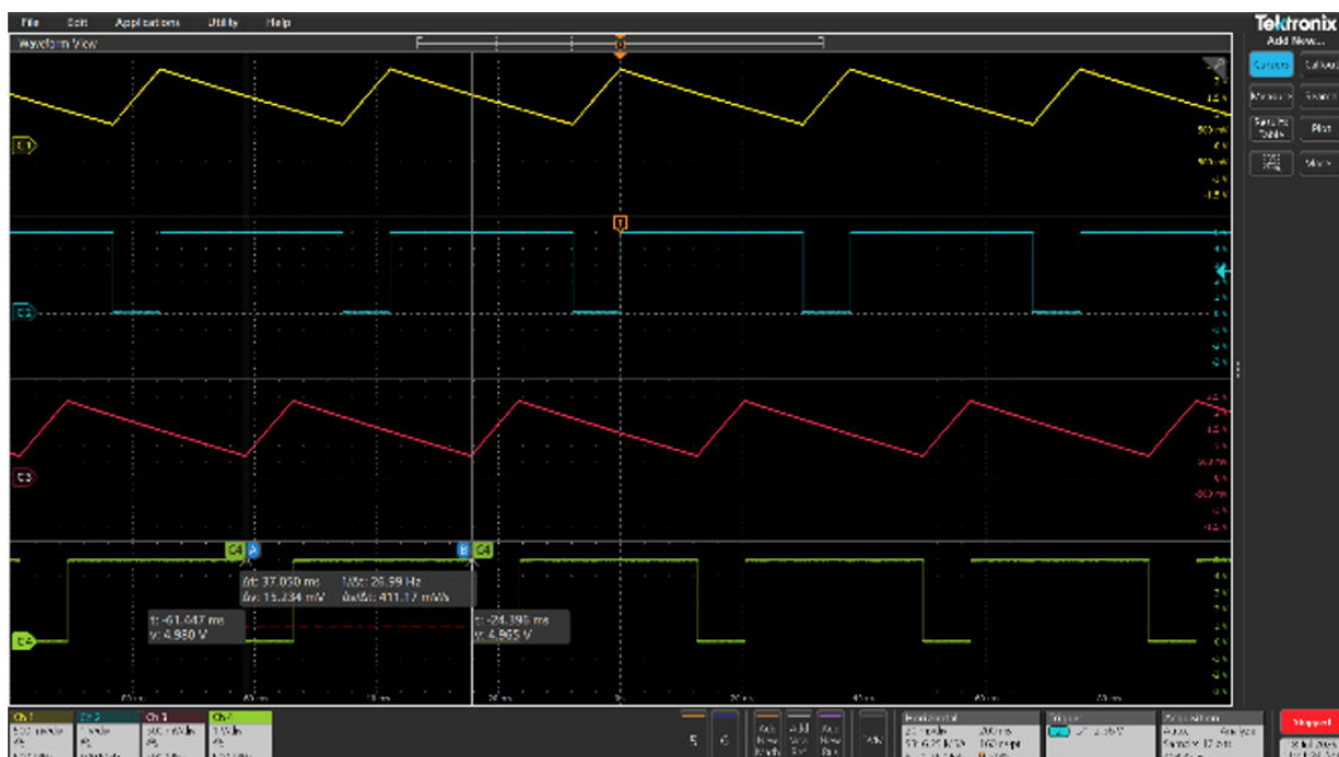
Figure 24. RS_LDO2 without Wi_LDO2 for VO2 output (VO2= 5V F=26.99Hz)
