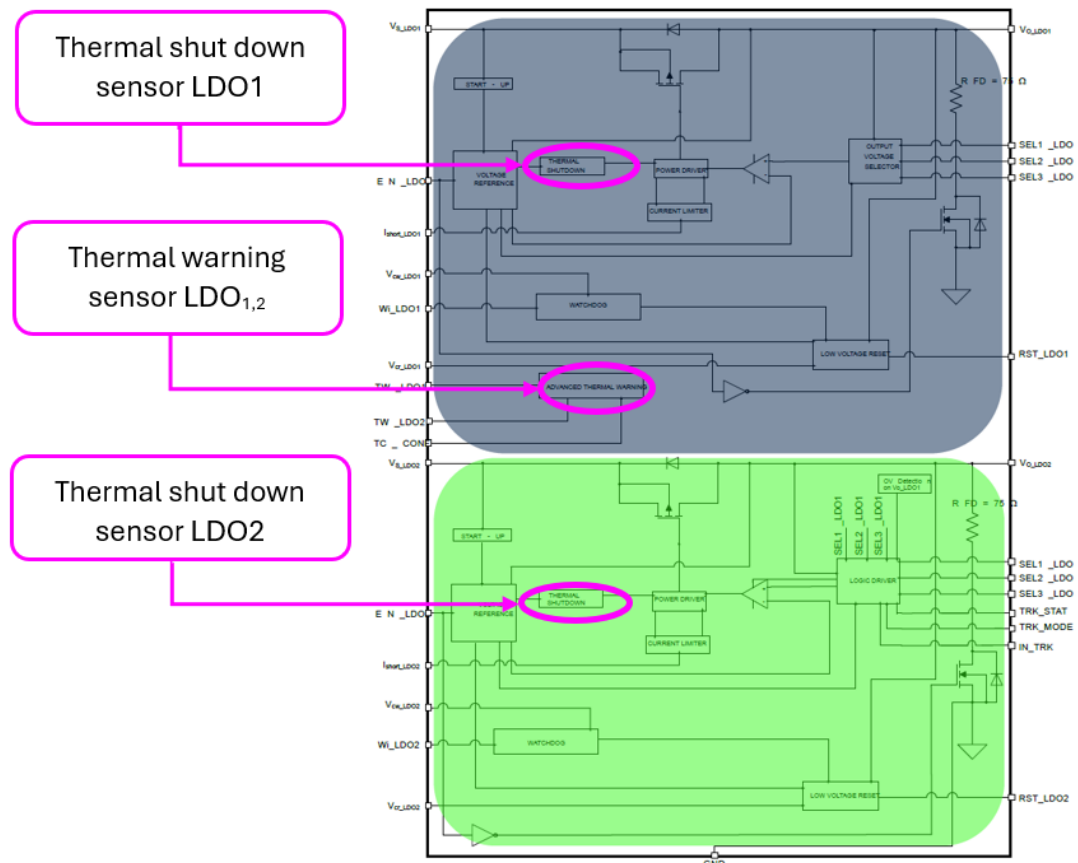
Figure 13. LDO1,2 thermal clusters
