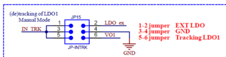
Figure 15. IN_TRK pin
