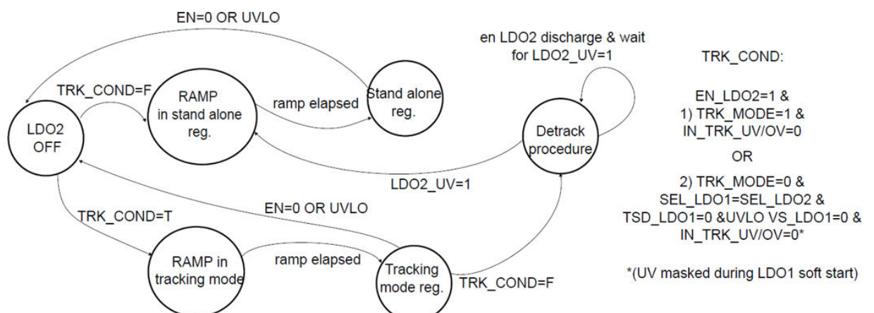
Figure 17. Tracking mode state machine
