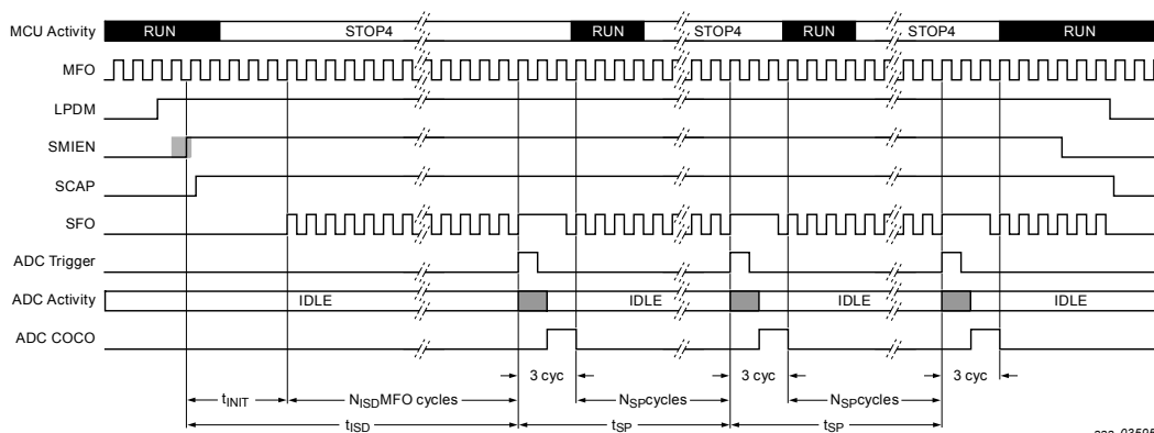
Figure 48. Low power direct measurement protocol
