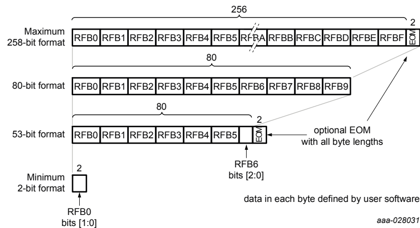
Figure 30. Data frame formats
