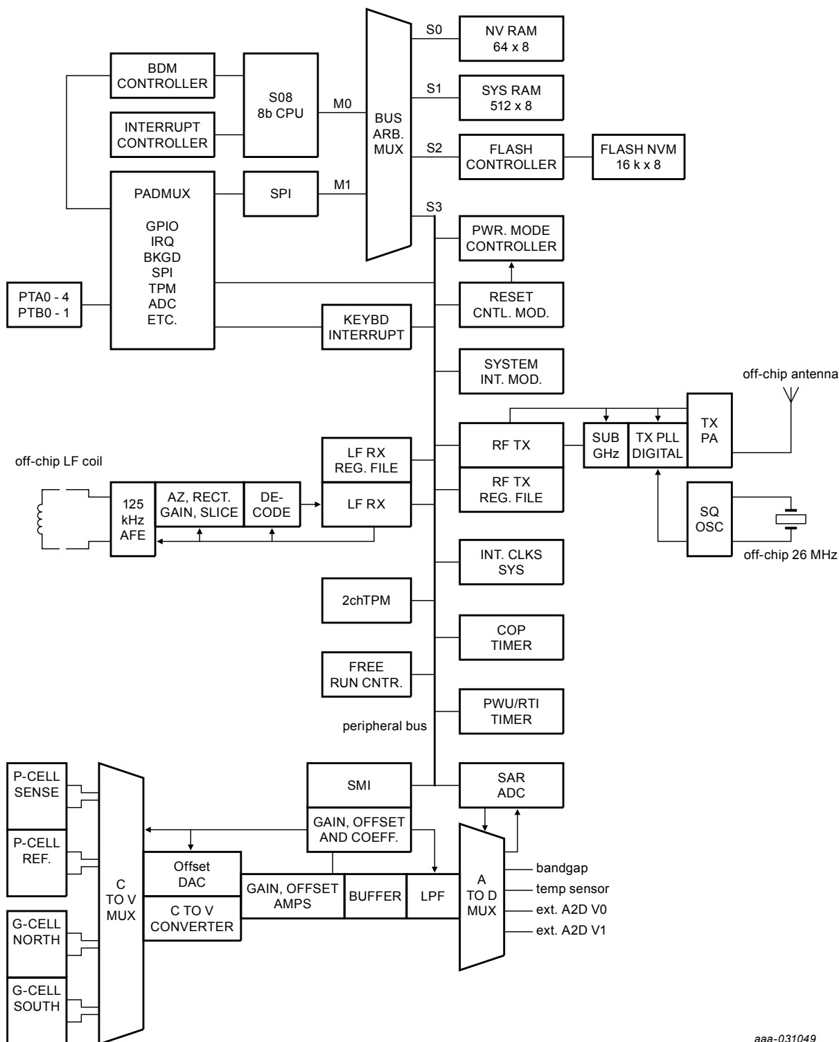
Figure 2. Block diagram
