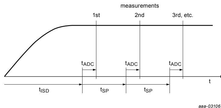
Figure 47. Initial and subsequent settling time protocol example at maximum times
