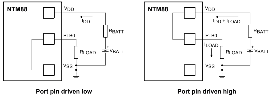
Figure 58. Battery check circuit
