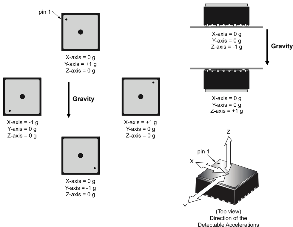
Figure 4. NTM88 orientation at rest.
