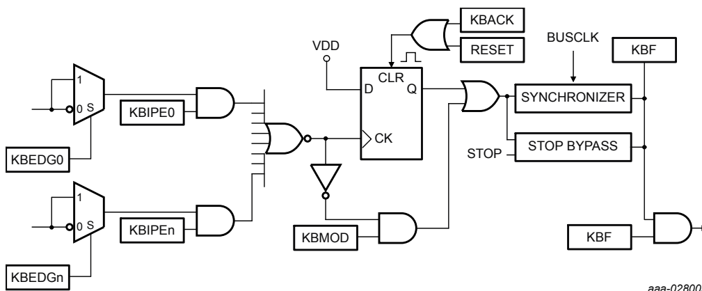
Figure 15. KBI block diagram
