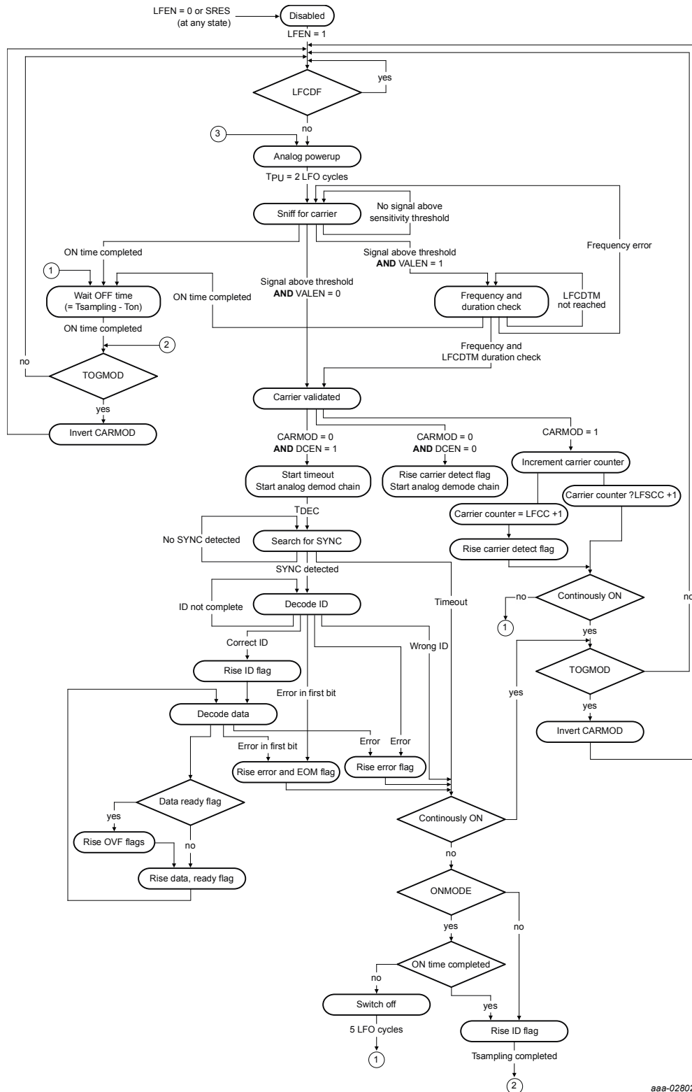
Figure 20. NTM88 LFR state machine diagram
