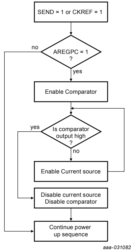
Figure 38. Pre-charge diagram
