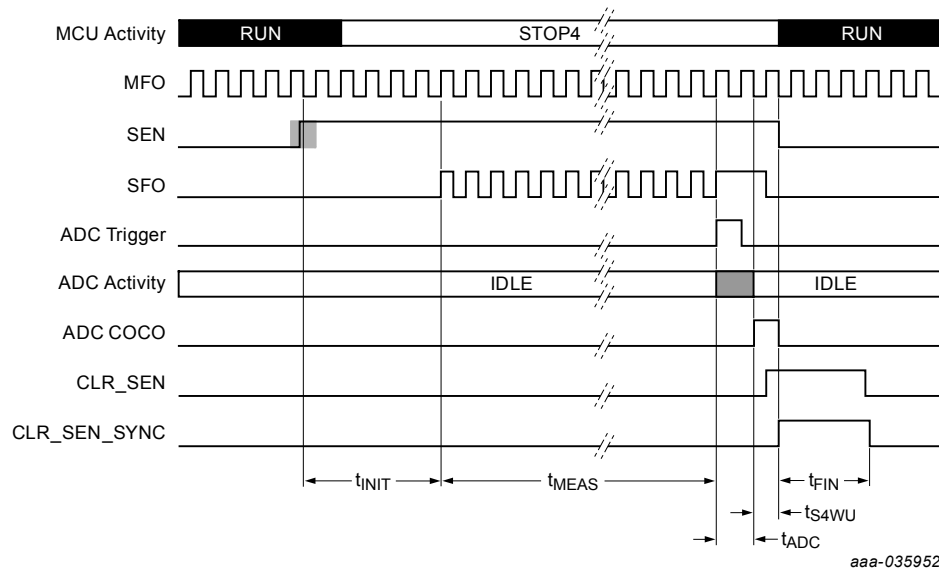
Figure 45. Automatic measurement protocol
