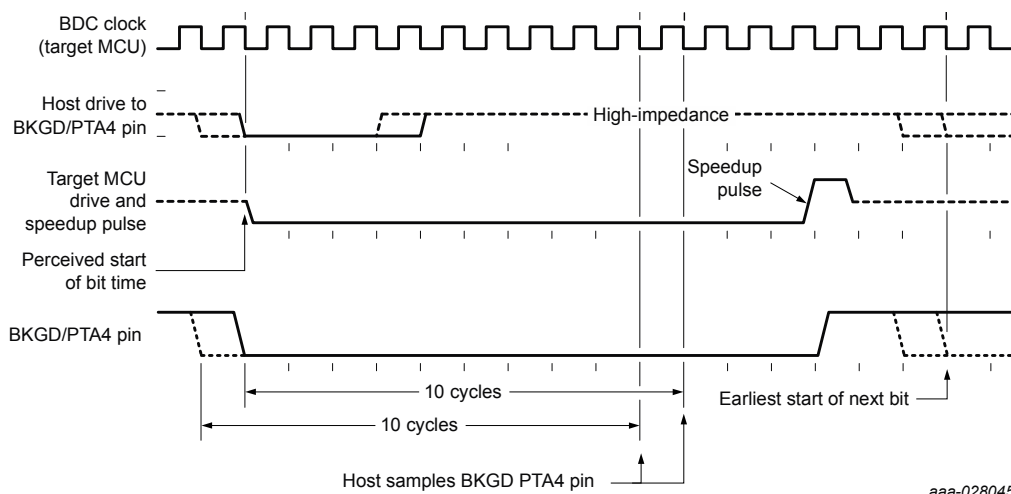
Figure 10. BDM target-to-host serial bit timing (Logic 0)
