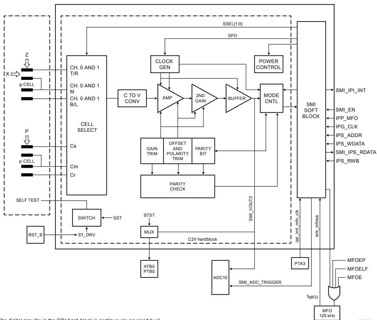
Figure 44. Sensor measurement interface block diagram
