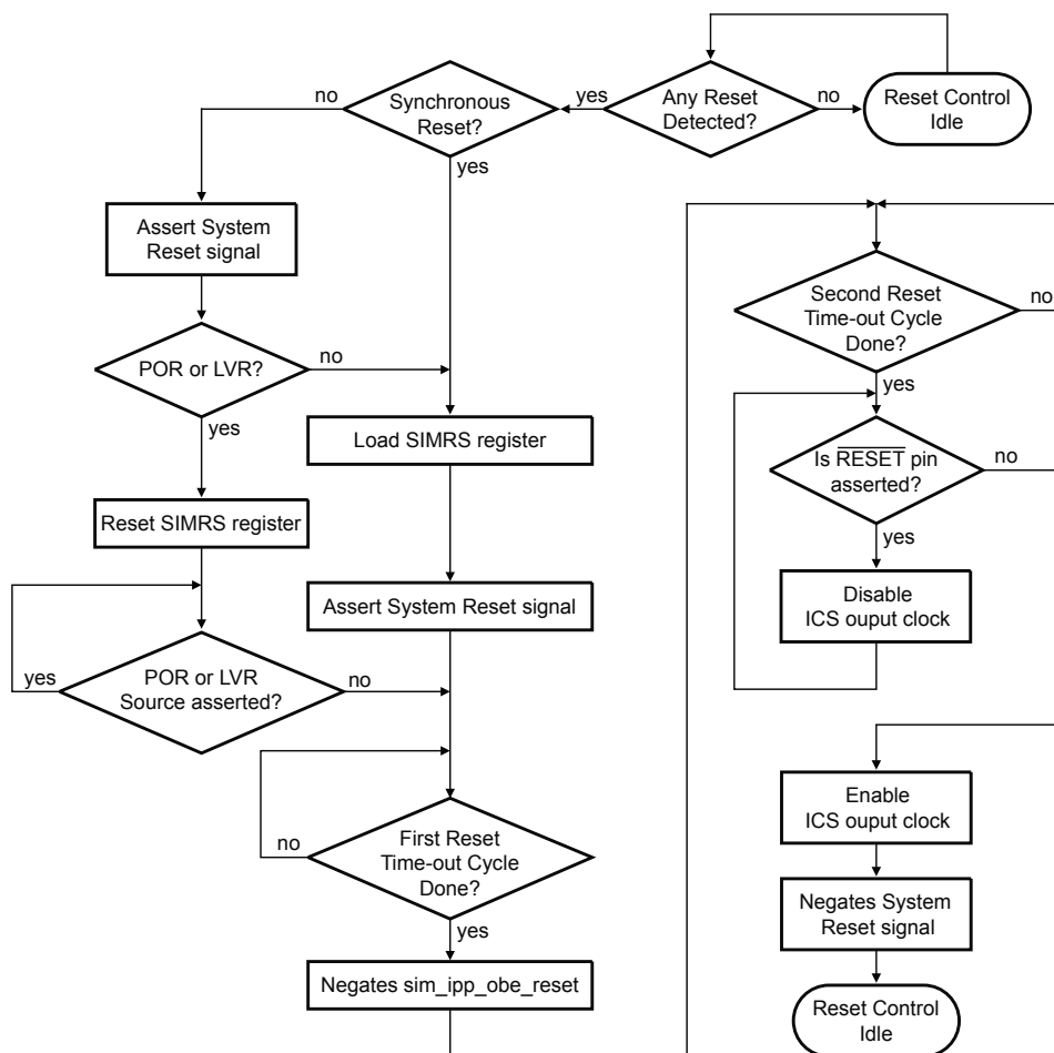
Figure 50. SIM reset exit diagram
