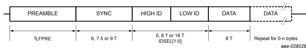
Figure 28. Telegram format (carrier preamble)
