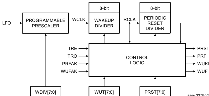
Figure 18. Periodic wake-up timer block diagram
