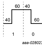
Figure 23. Definition of duty cycle of 40 %
