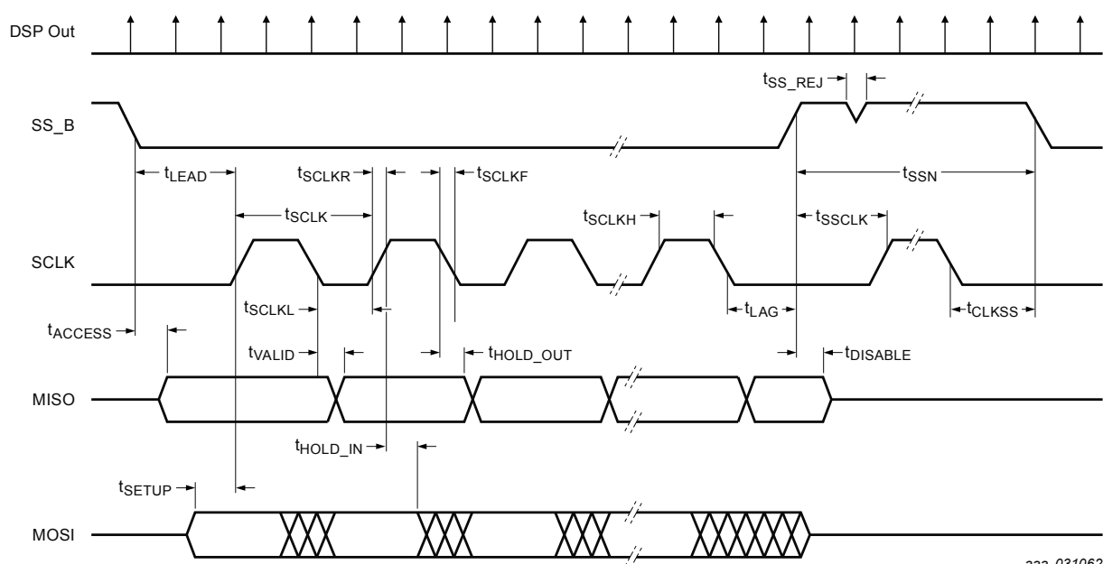
Figure 43. SPI signal timing diagram
