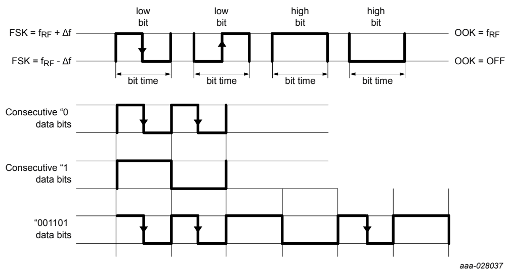
Figure 36. Bi-Phase data bit encoding (POL = 0)
