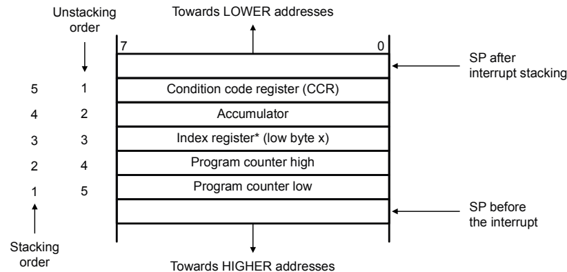
Figure 11. Interrupt stack frame
