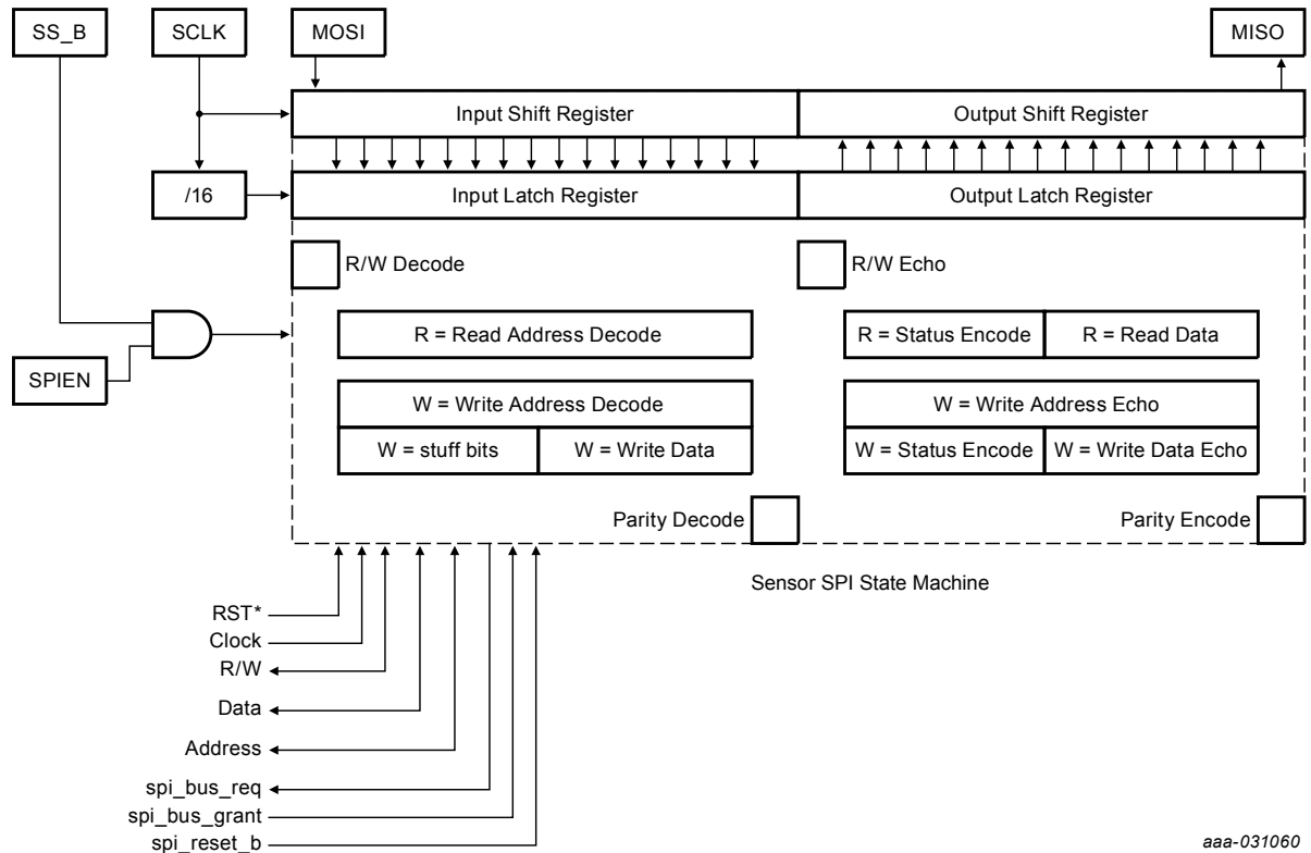
Figure 41. Sensor SPI state machine
