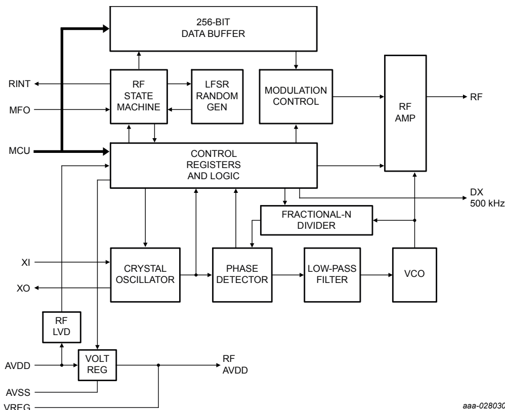
Figure 29. Radio frequency module block diagram
