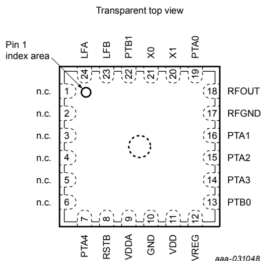
Figure 3. NTM88 QFN package pinout
