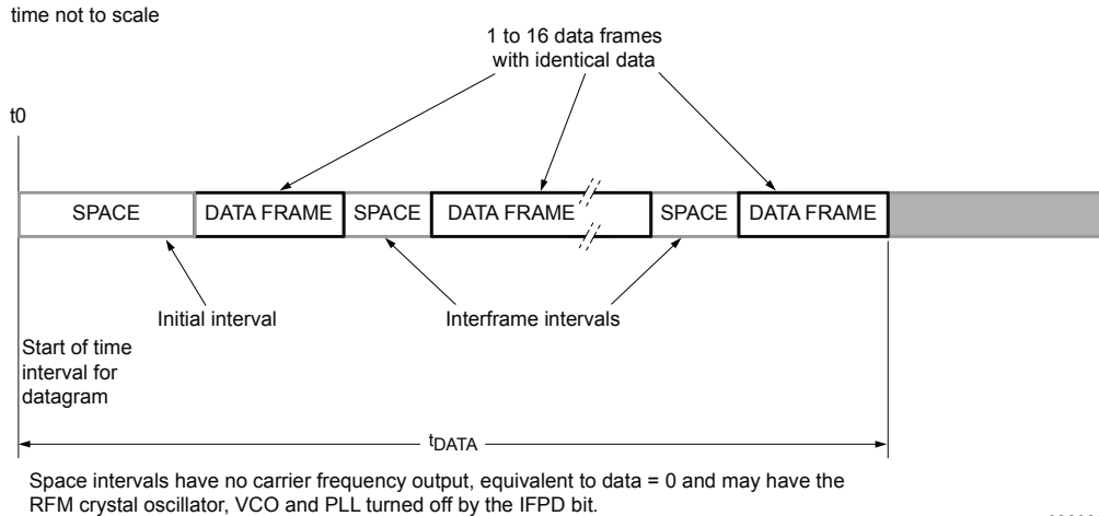
Figure 31. Radio frequency transmission randomization
