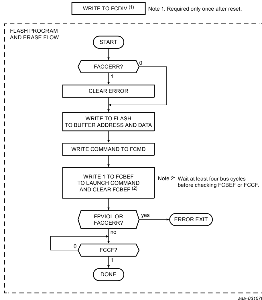
Figure 55. FMC program and erase command flow diagram
