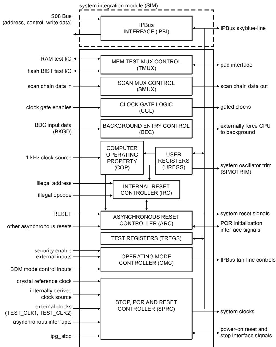
Figure 49. System integration module block diagram
