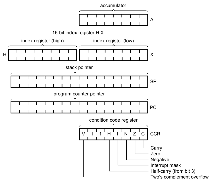
Figure 5. CPU registers
