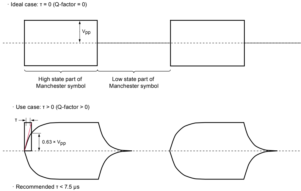
Figure 26. LF envelope filtering
