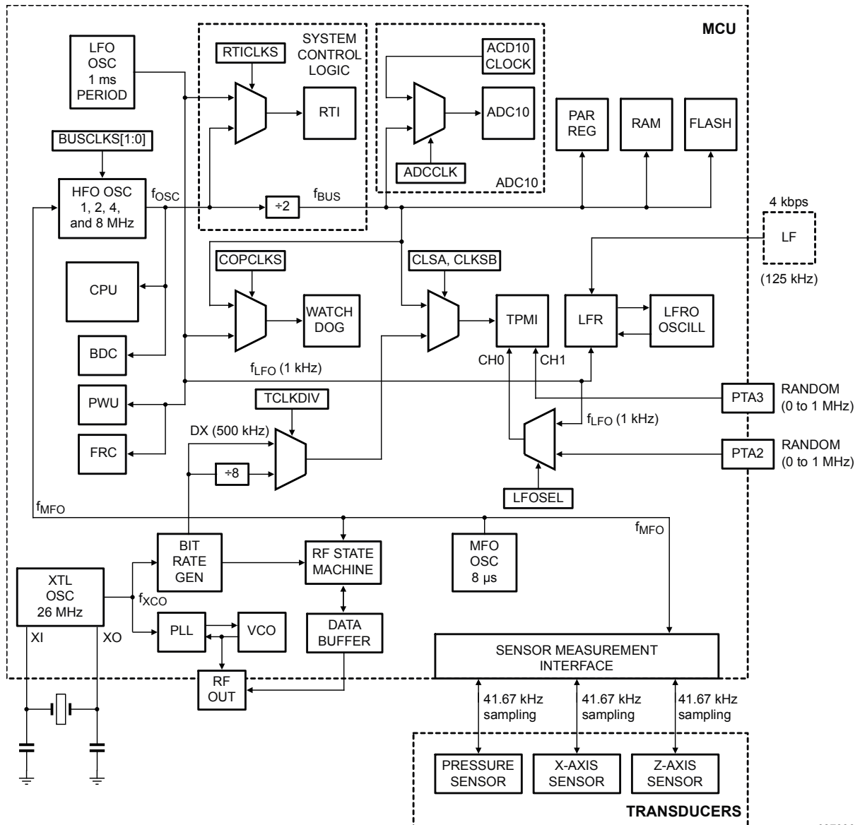
Figure 12. Clock distribution
