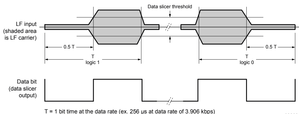
Figure 21. Manchester encoded datagram for LFPOL = 0
