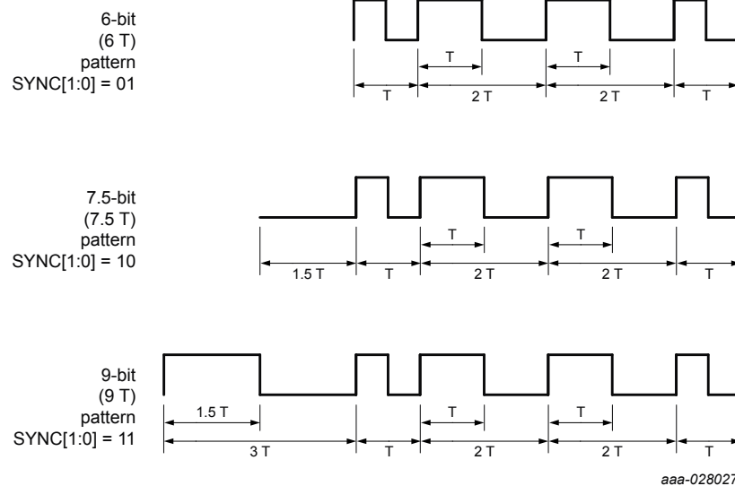
Figure 27. SYNC patterns
