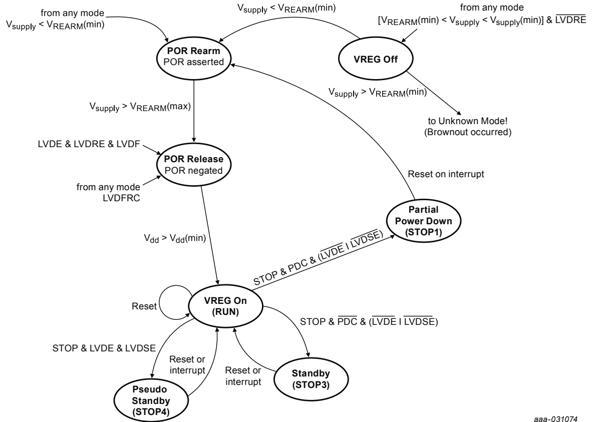
Figure 53. Power management controller state transition diagram
