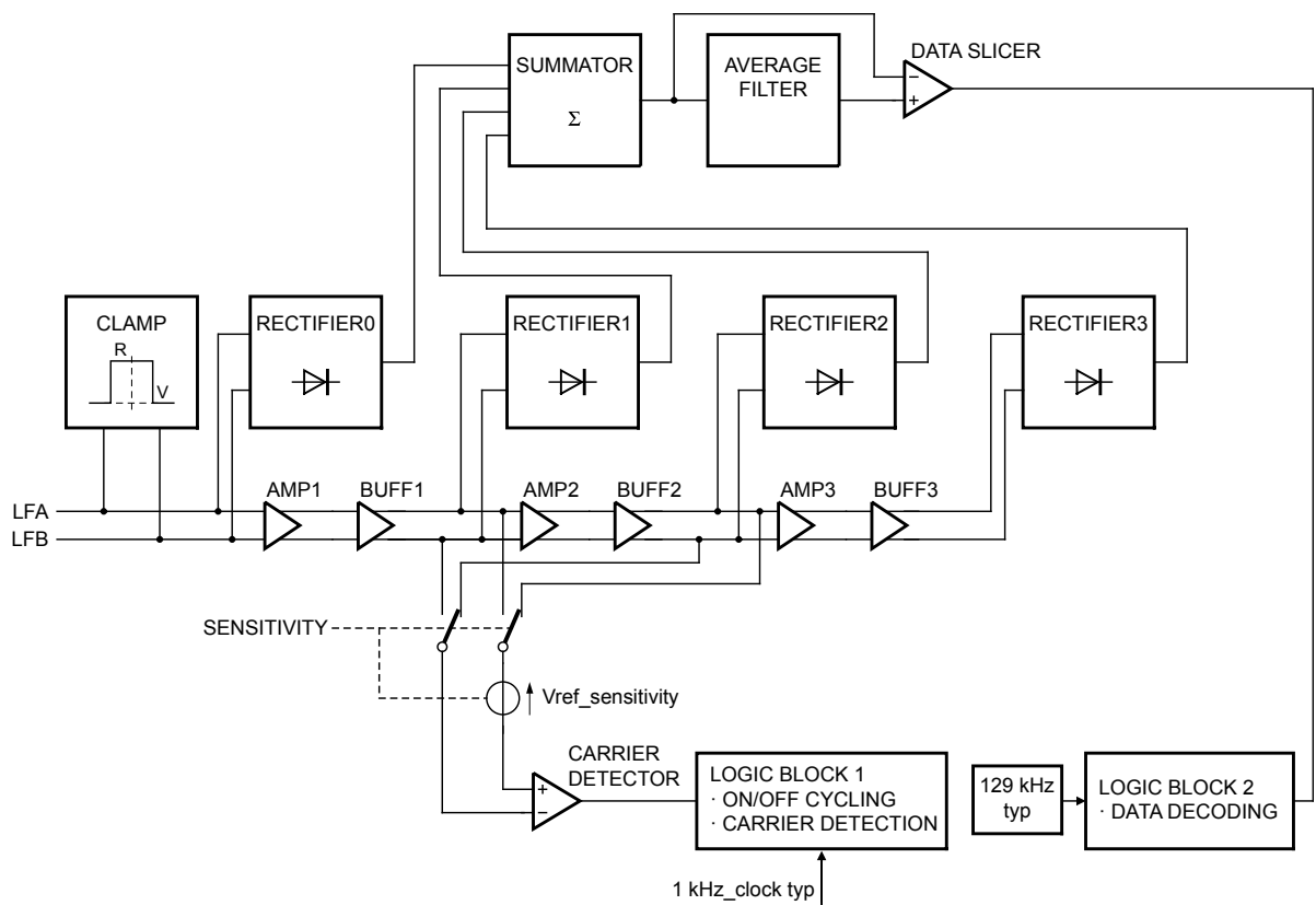
Figure 19. Block diagram
