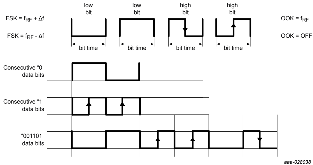
Figure 37. Bi-Phase data bit encoding (POL = 1)
