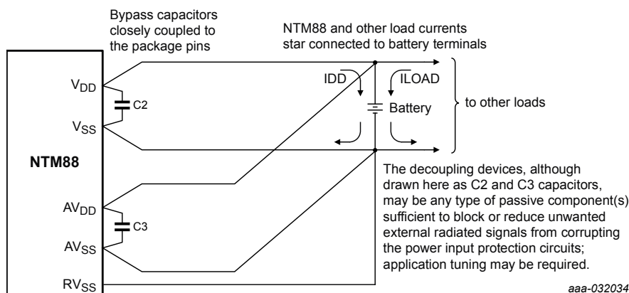
Figure 61. Recommended power supply connections
