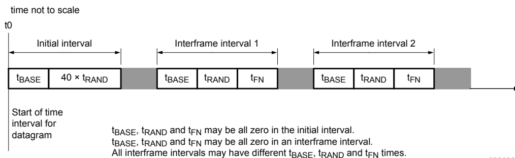
Figure 32. Radio frequency transmission initial and interframe time intervals
