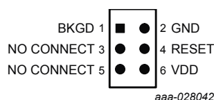
Figure 7. BDM tool connector
