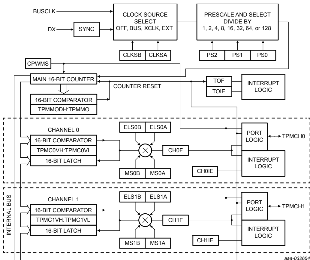
Figure 17. Timer pulse-width block diagram
