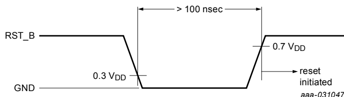
Figure 62. RESET pin timing
