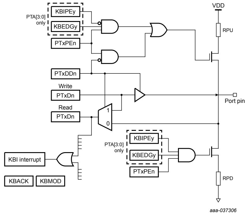
Figure 14. General purpose I/O logic
