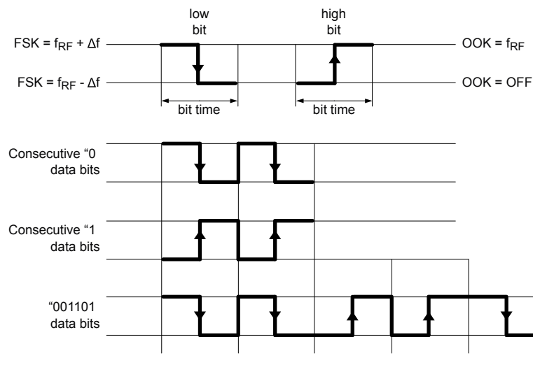
Figure 35. Manchester data bit encoding (POL = 1)
