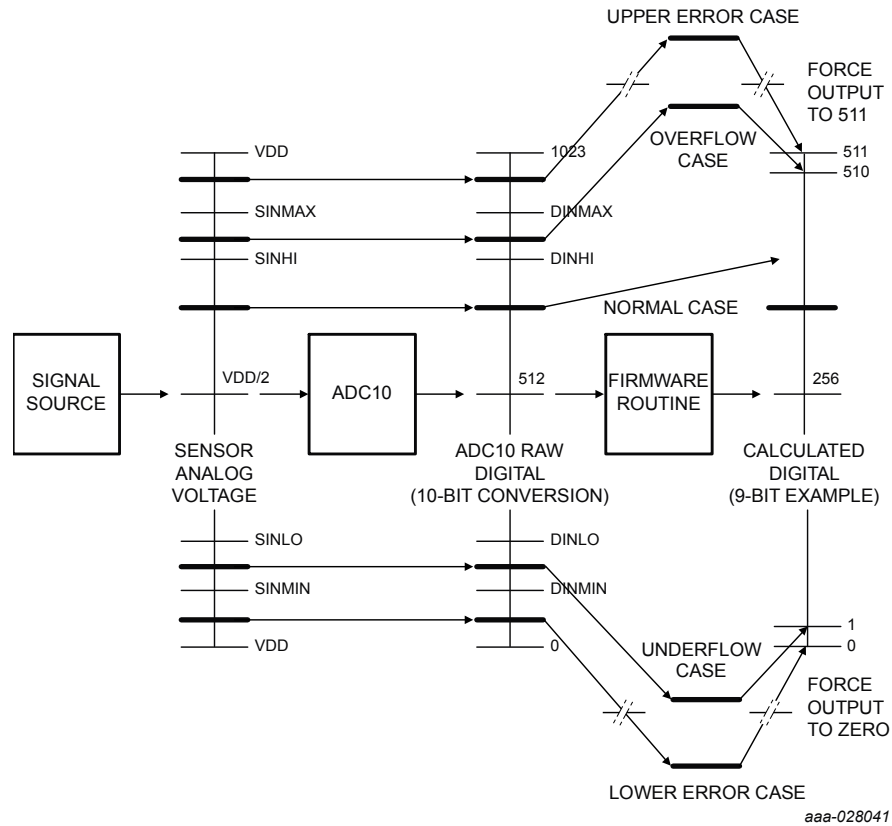
Figure 1. Measurement signal range definitions
