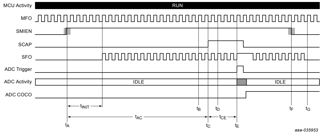
Figure 46. Direct measurement protocol
