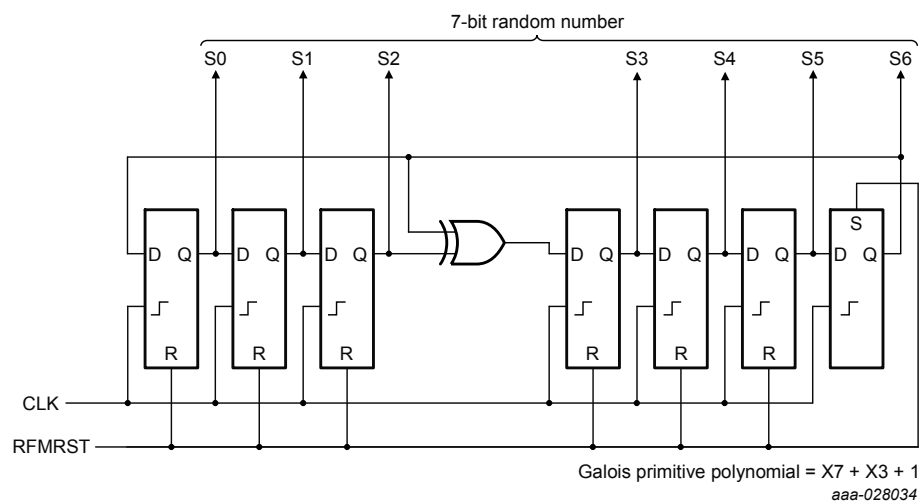
Figure 33. LFSR implementation
