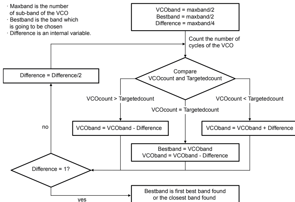
Figure 39. VCO calibration state machine
