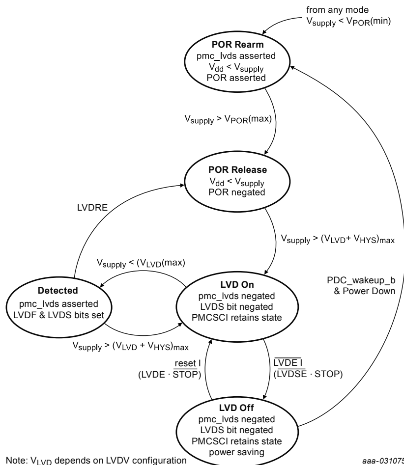
Figure 54. Power management controller low voltage detection transitions state diagram
