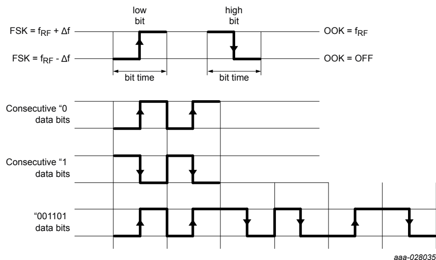
Figure 34. Manchester data bit encoding (POL = 0)
