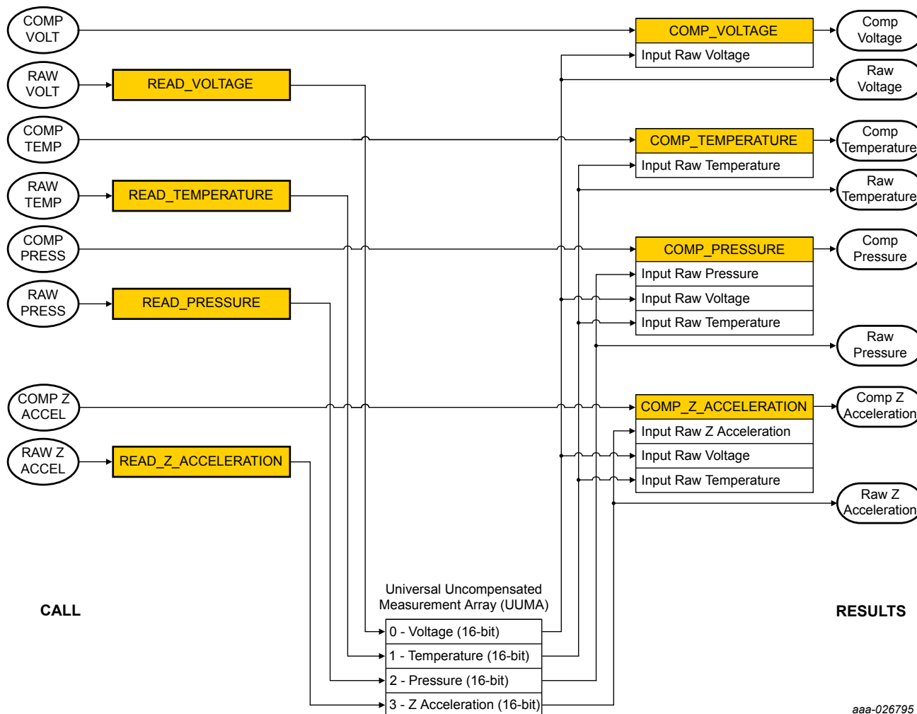
Figure 59. Example single axis accelerometer data flow for measurements
