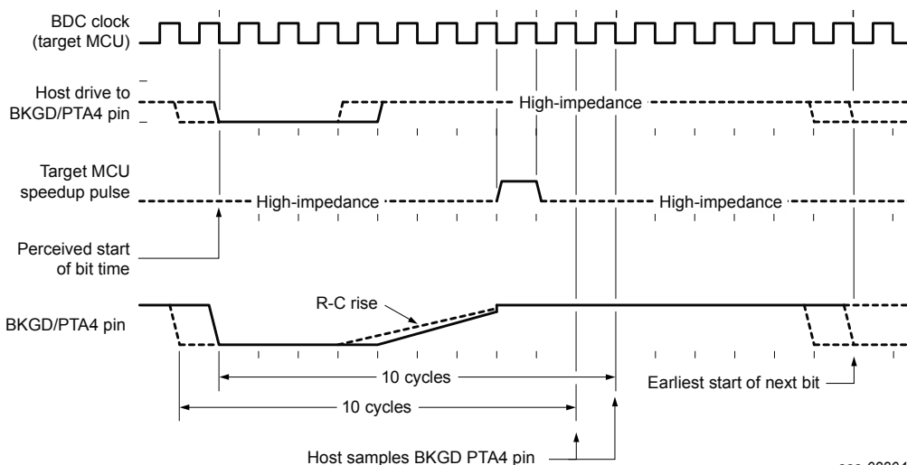
Figure 9. BDC target-to-host serial bit timing (Logic 1)
