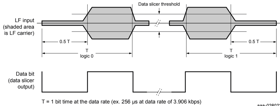
Figure 22. Manchester encoded datagram for LFPOL = 1
