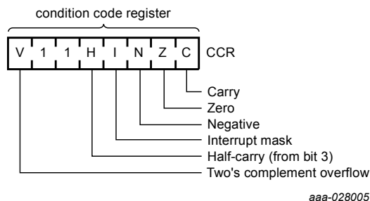
Figure 6. Condition code register
