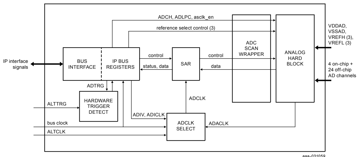
Figure 40. Analog to digital converter block diagram
