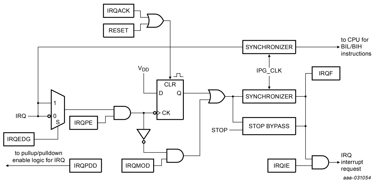
Figure 16. External interrupt logic
