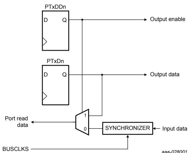
Figure 13. General purpose I/O block diagram
