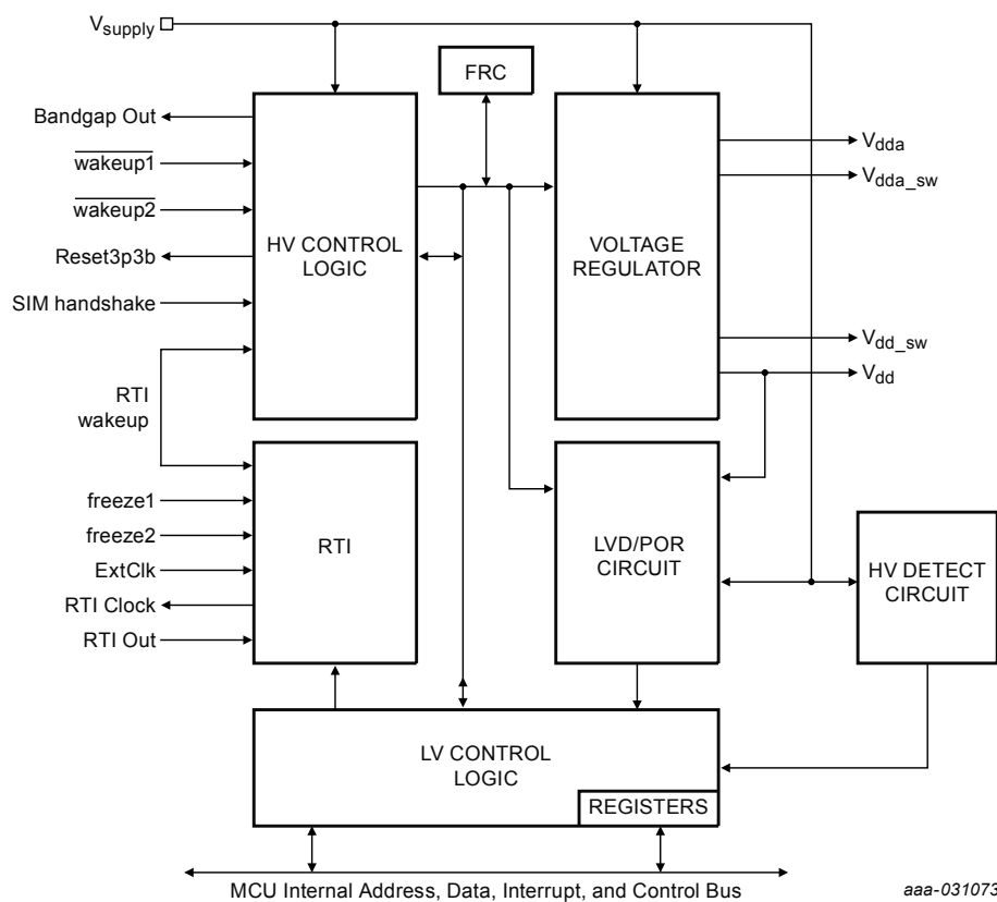
Figure 52. Power management controller module block diagram
