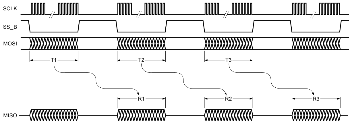
Figure 42. SPI message response protocol
