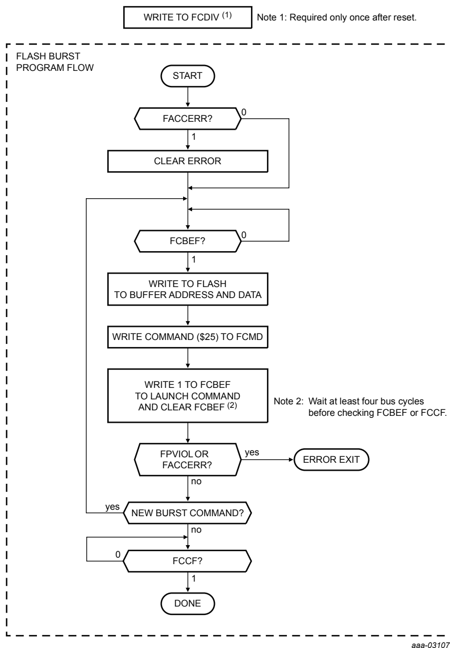
Figure 56. FMC burst program flow diagram
