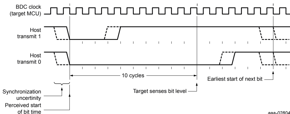
Figure 8. BDC host-to-target serial bit timing
