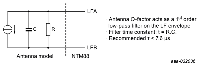
Figure 25. Antenna Q-factor equivalent model for the LF envelope
