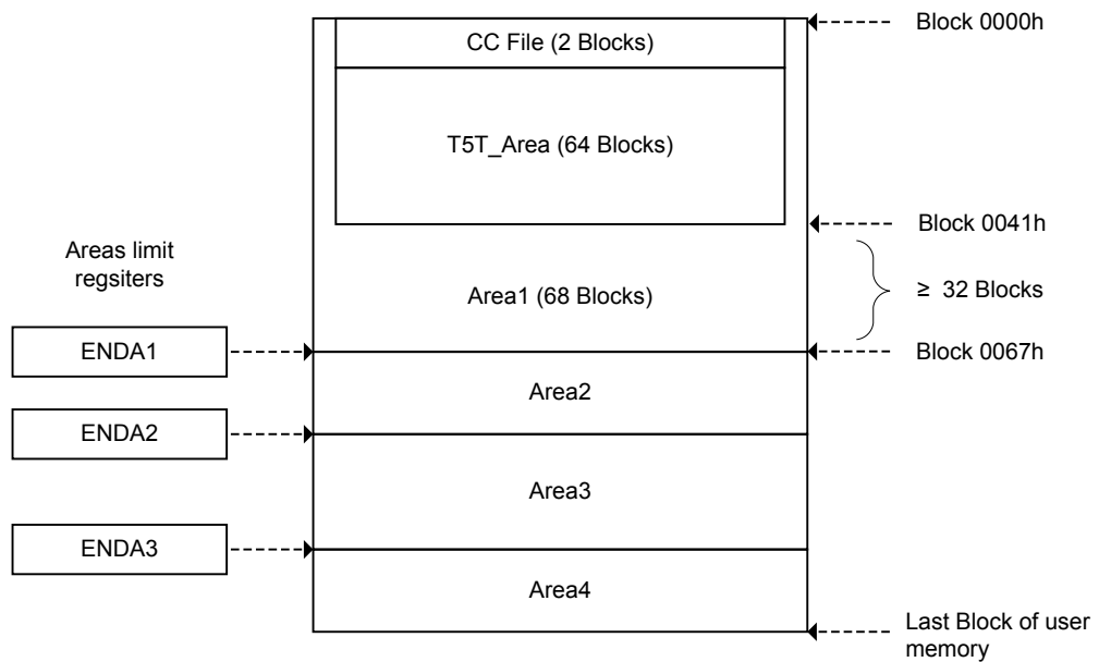
Figure 1. ST25DV-I2C, ST25TV16K and ST25TV64K user memory
