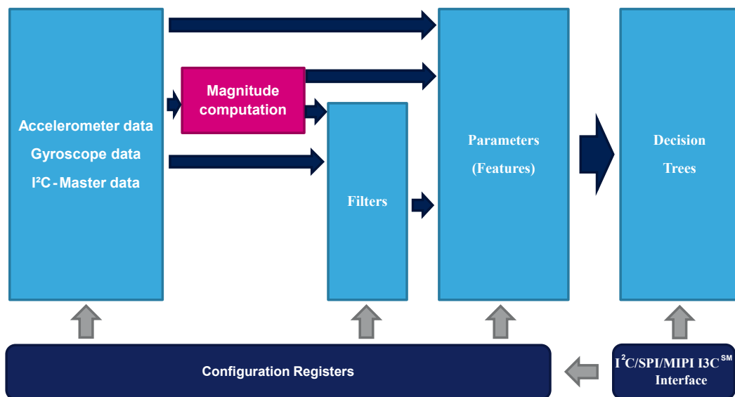
Figure 2. Machine learning core in the ASM330LHHX
