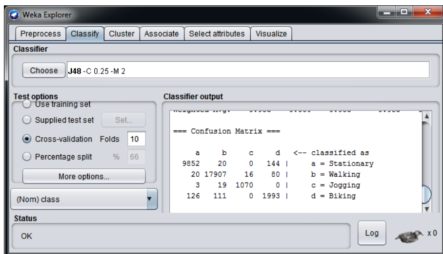
Figure 52. Confusion matrix
