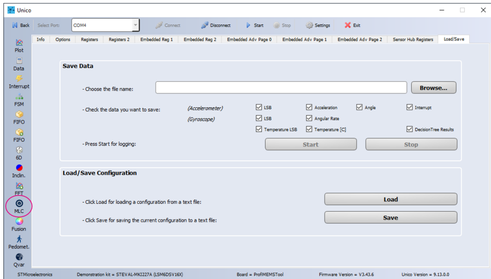
Figure 21. Unico GUI
