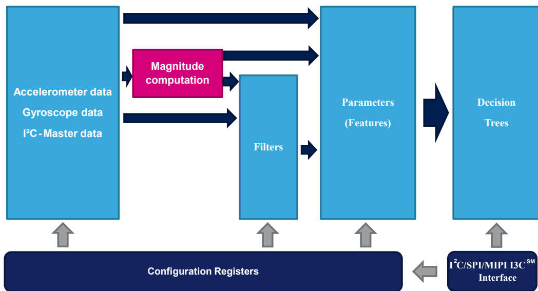
Figure 2. Machine learning core in the LSM6DSV16X
