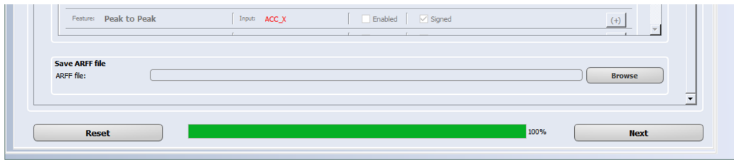
Figure 33. ARFF generation
