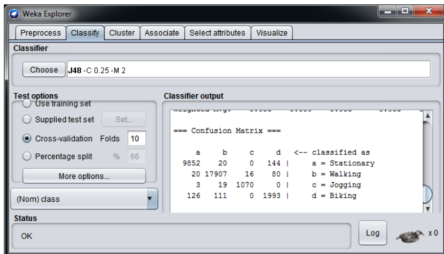
Figure 48. Confusion matrix
