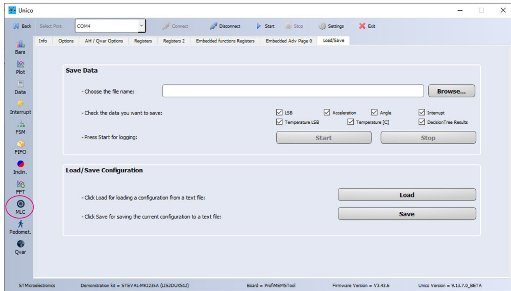
Figure 20. Unico GUI
