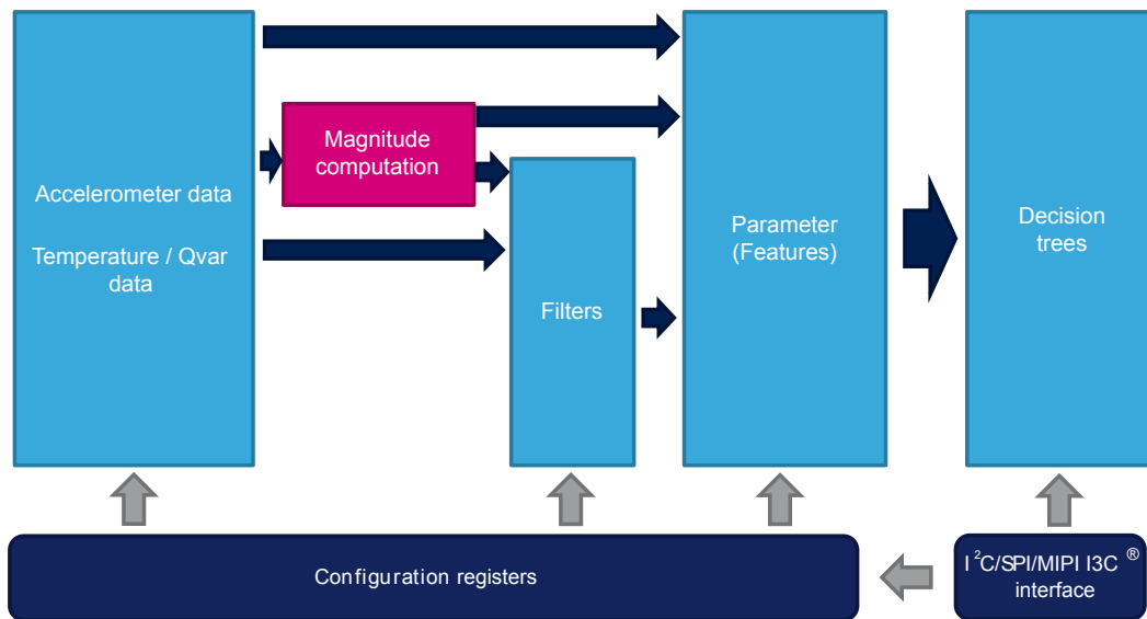
Figure 2. Machine learning core in the LIS2DUXS12
