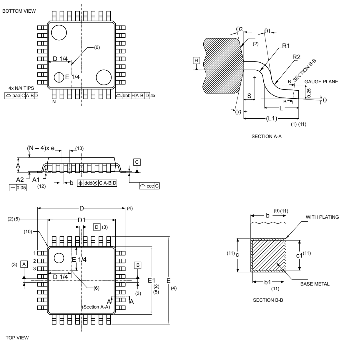
Figure 45. LQFP32- Outline
