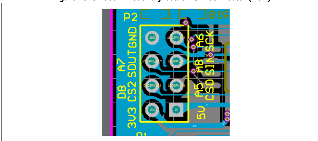
Figure 13. SPC56L-Discovery board - SPI connector (PCB)
