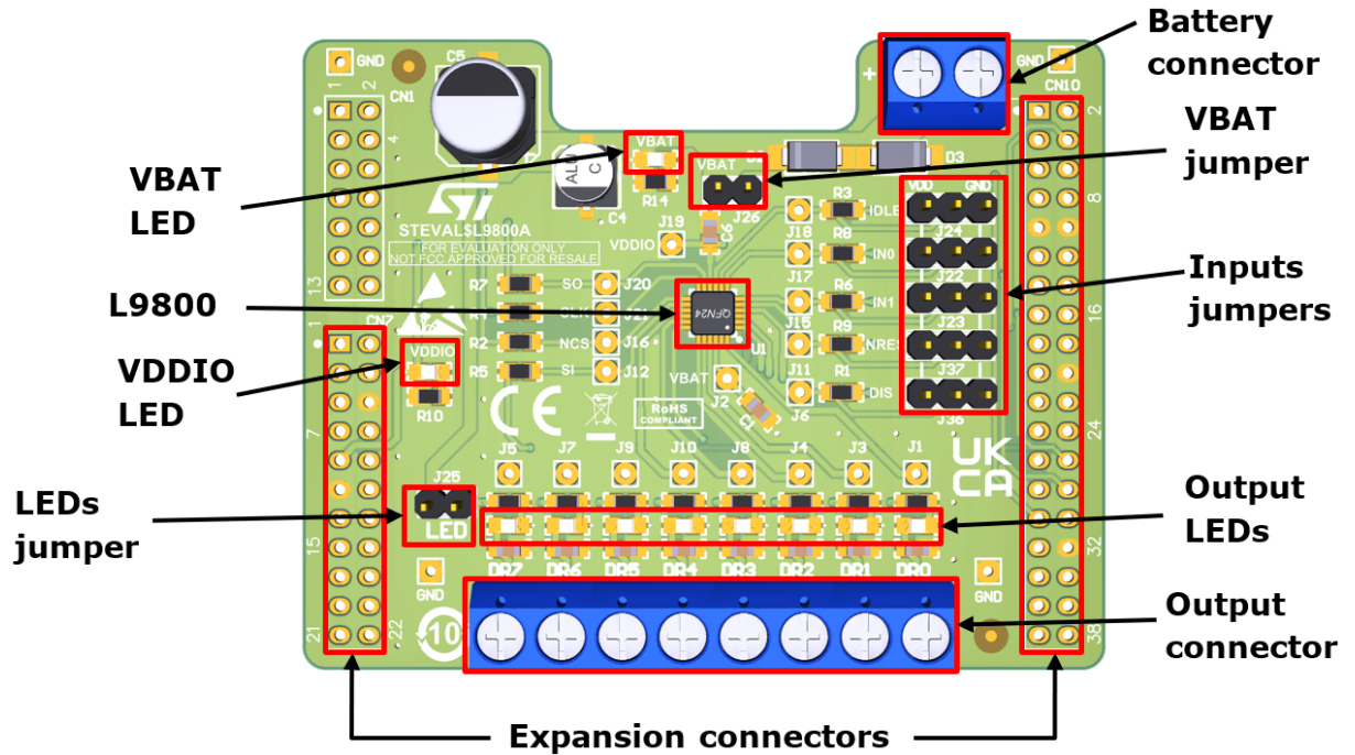
Figure 3. Evaluation board main components and connectors
