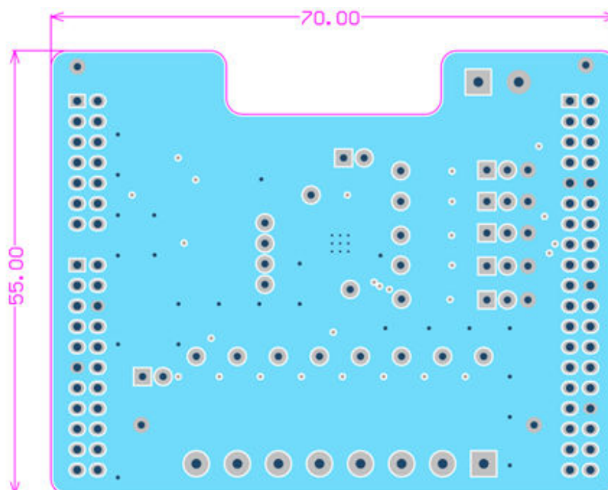
Figure 7. Inner 2
