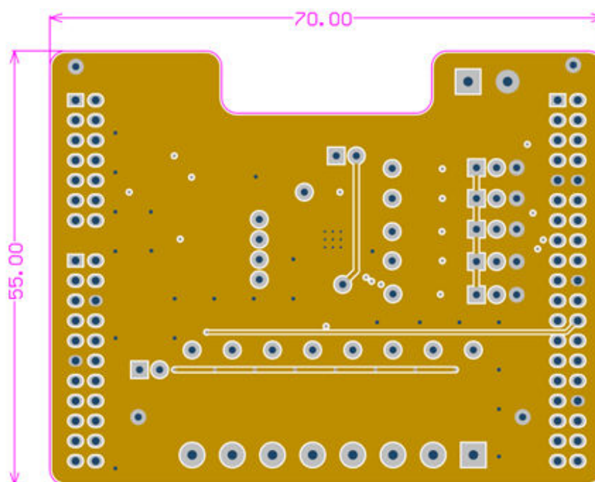
Figure 6. Inner 1
