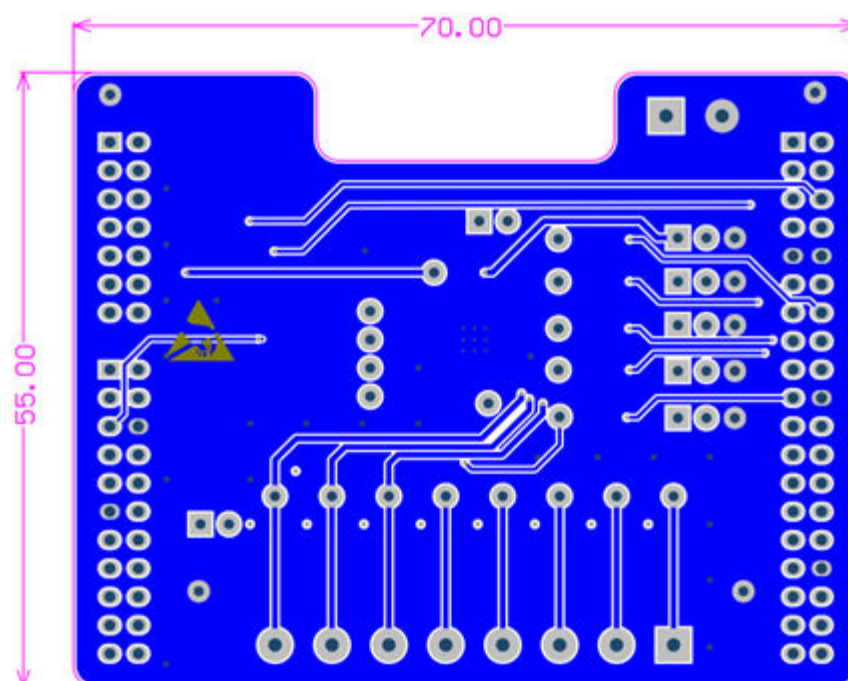
Figure 8. Assembly bottom
