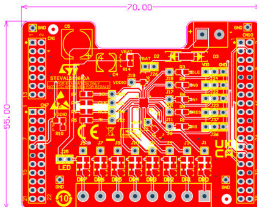
Figure 5. Assembly top
