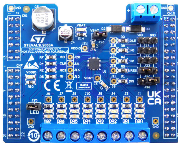
Figure 1. STEVAL-L9800 board
