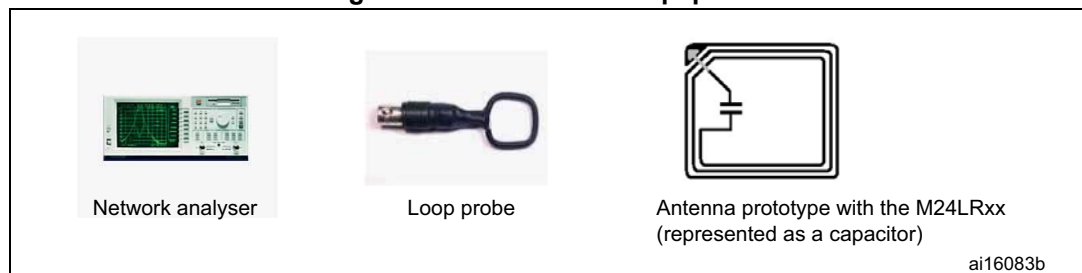
Figure 19. Measurement equipment
