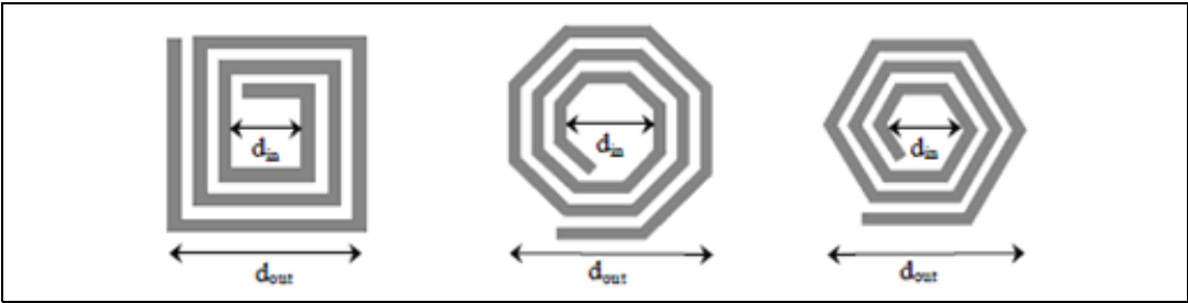
Figure 11. Square antennas
