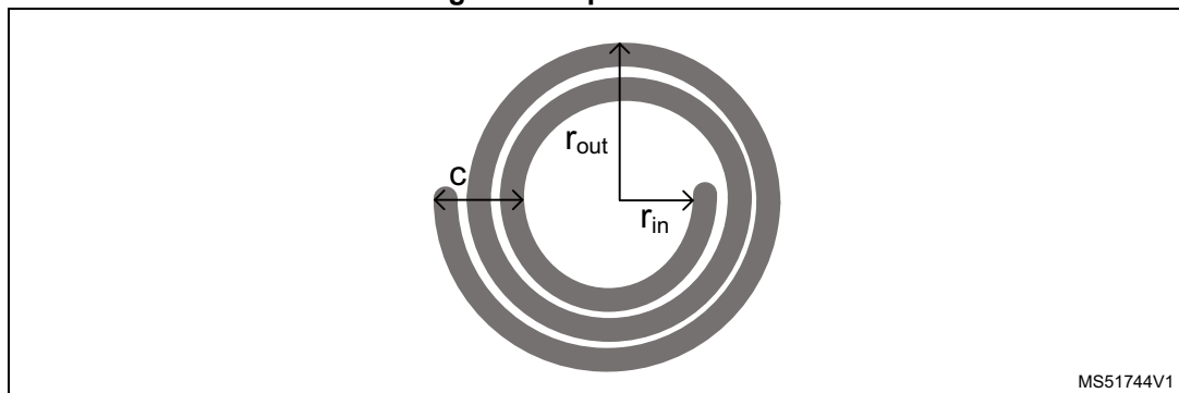
Figure 10. Spiral antenna
