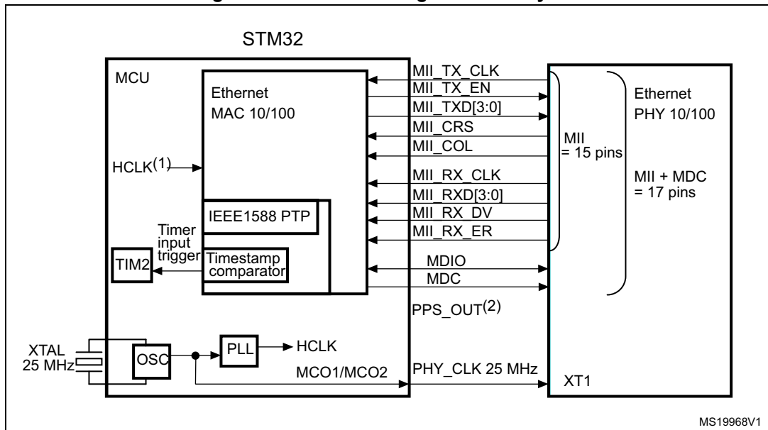
Figure 89. MII mode using a 25 MHz crystal
