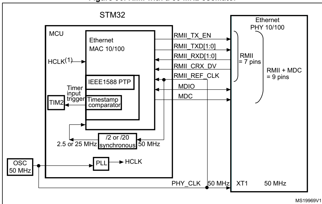
Figure 90. RMIi with a 50 MHz oscillator
