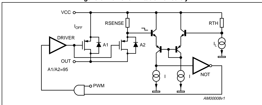
Figure 6. Current limitation circuitry
