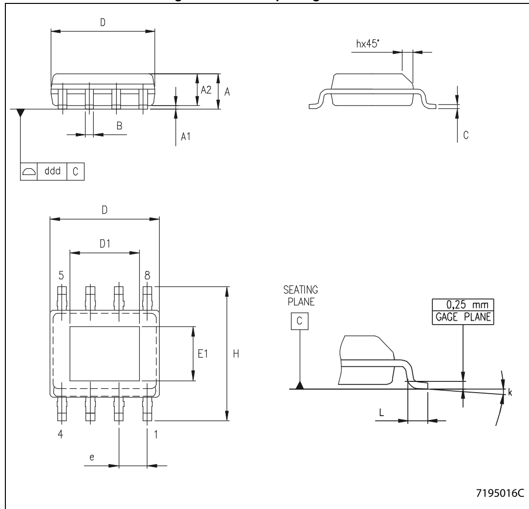
Figure 38. HSOP8 package outline
