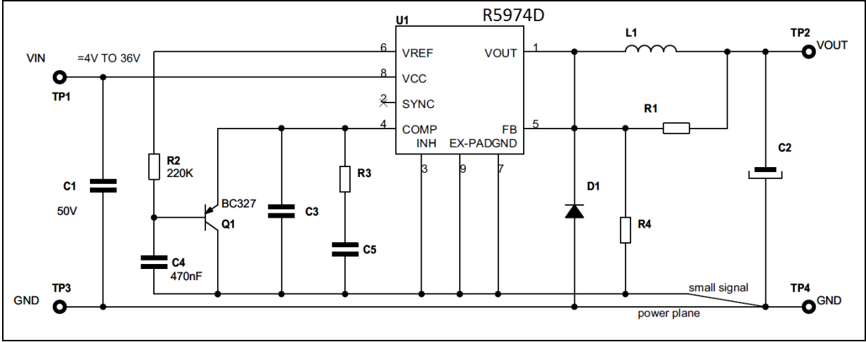
Figure 28. Soft-start network example
