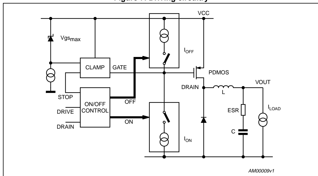
Figure 7. Driving circuitry
