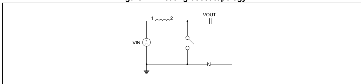
Figure 24. Floating boost topology
