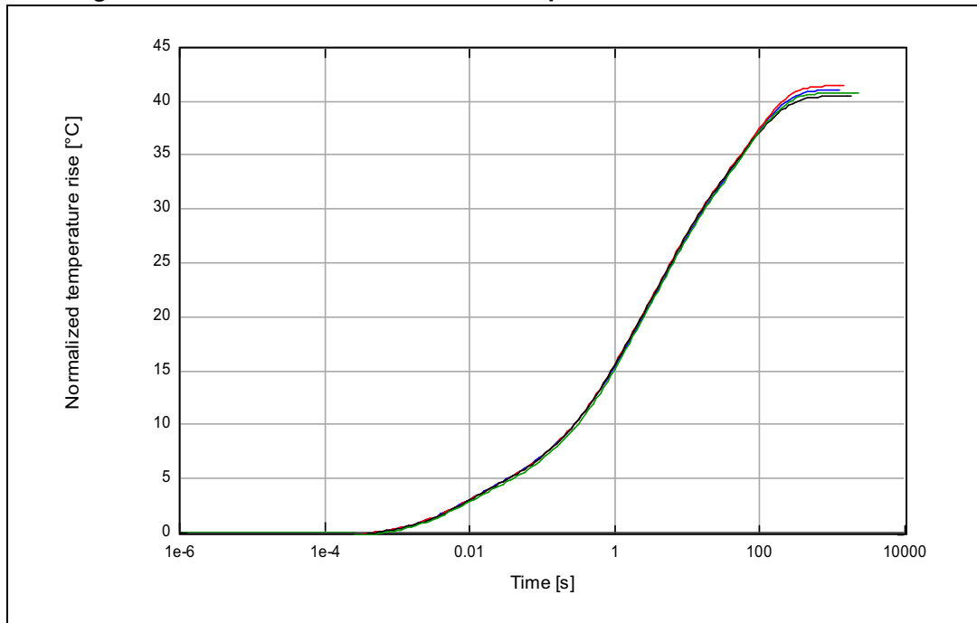
Figure 17. Measurement of the thermal impedance of the evaluation board
