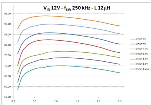
Figure 36. Efficiency vs. output current V_{IN} = 12\text{ V}
