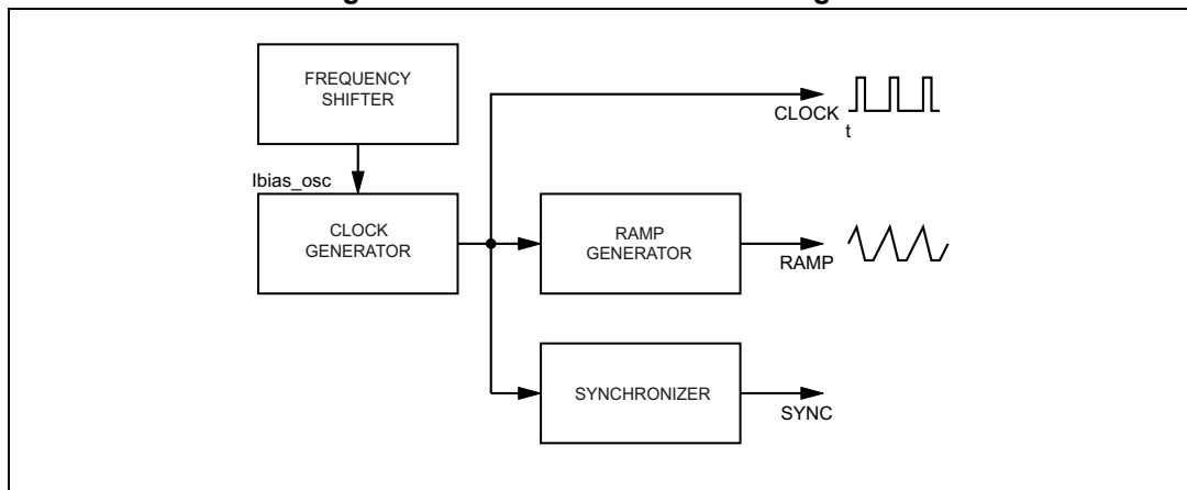
Figure 4. Oscillator circuit block diagram
