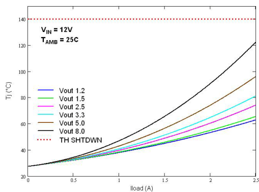
Figure 35. Junction temperature vs. output current V_{IN} = 12\text{ V}
