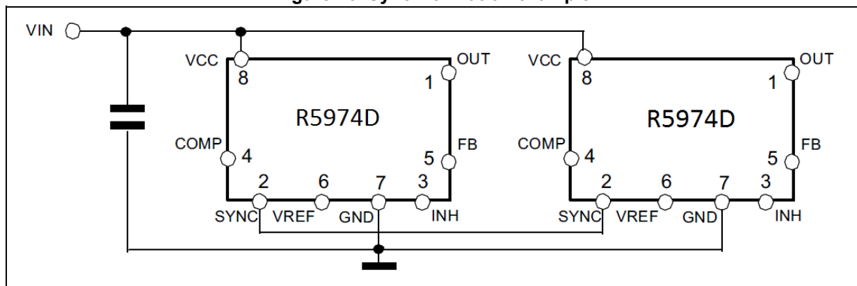
Figure 26. Synchronization example
