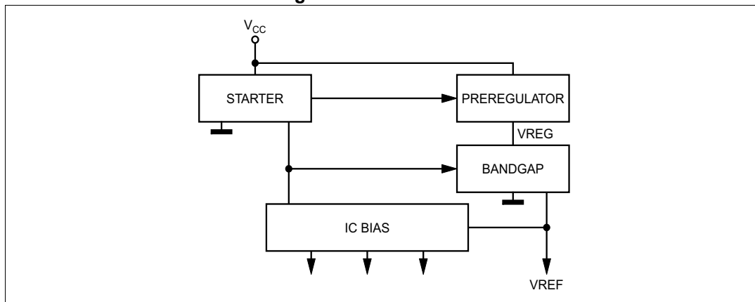
Figure 3. Internal circuit
