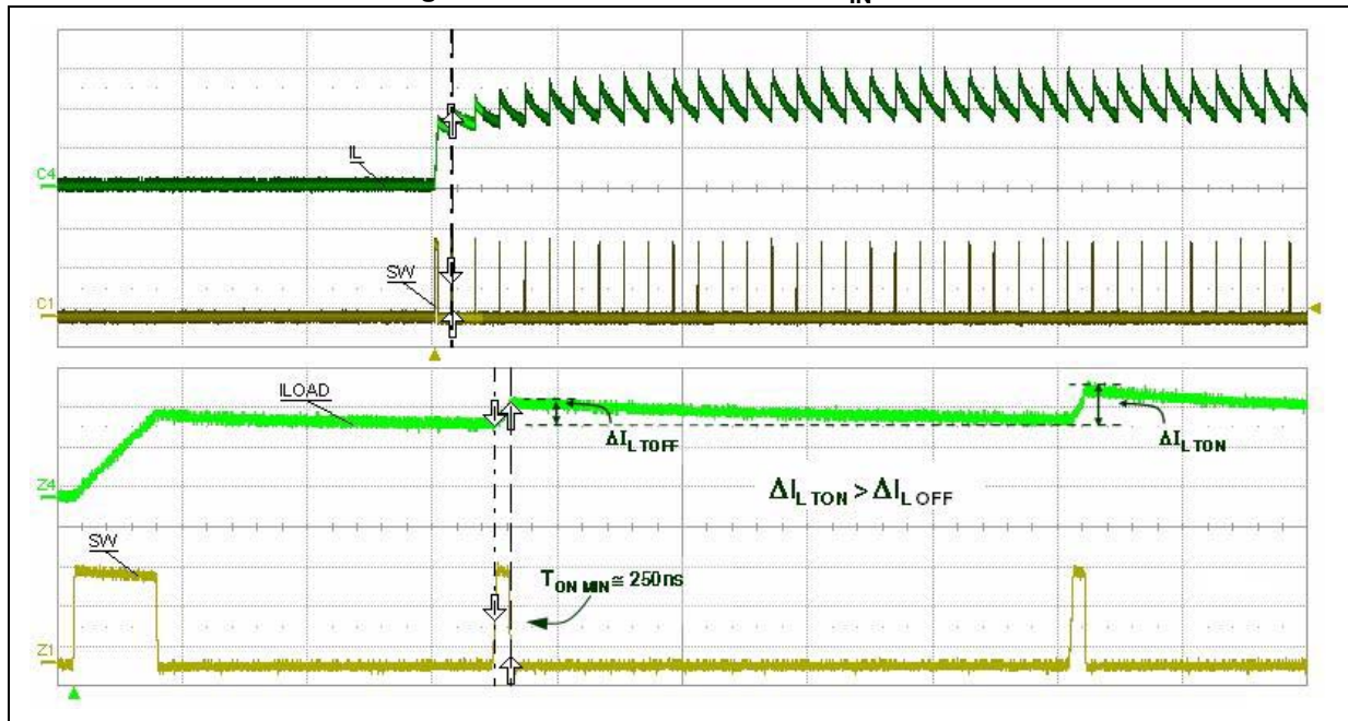
Figure 21. Short-circuit current V_{IN} = 36\text{ V}
