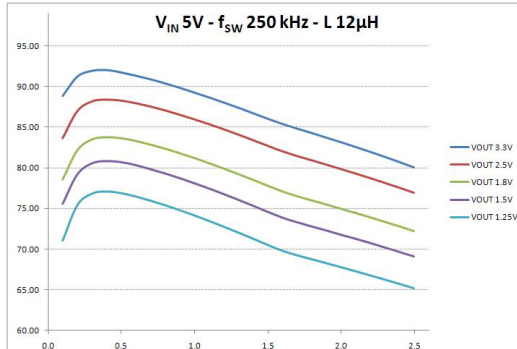
Figure 37. Efficiency vs. output current V_{IN} = 5\text{ V}
