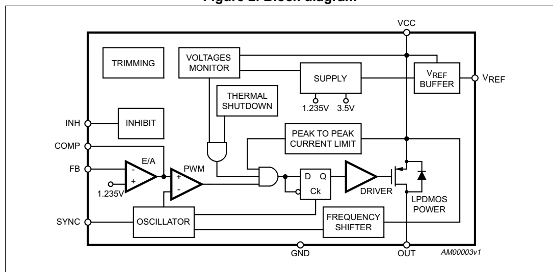
Figure 2. Block diagram
