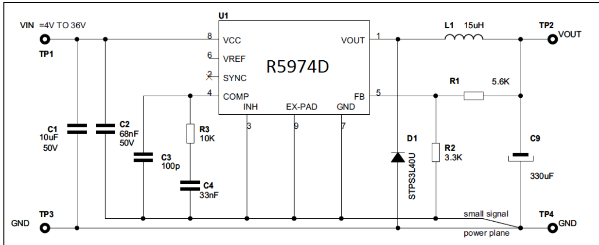
Figure 12. Application schematic
