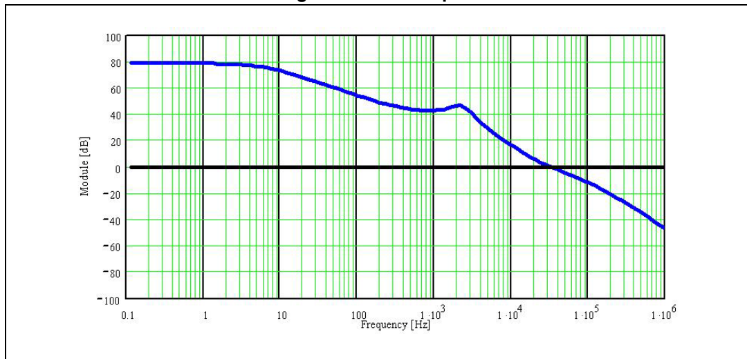
Figure 10. Module plot
