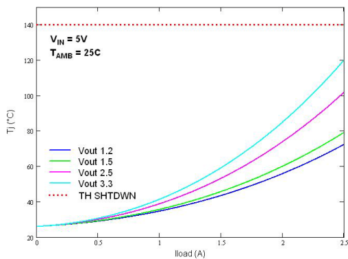
Figure 34. Junction temperature vs. output current V_{IN} = 5\text{ V}
