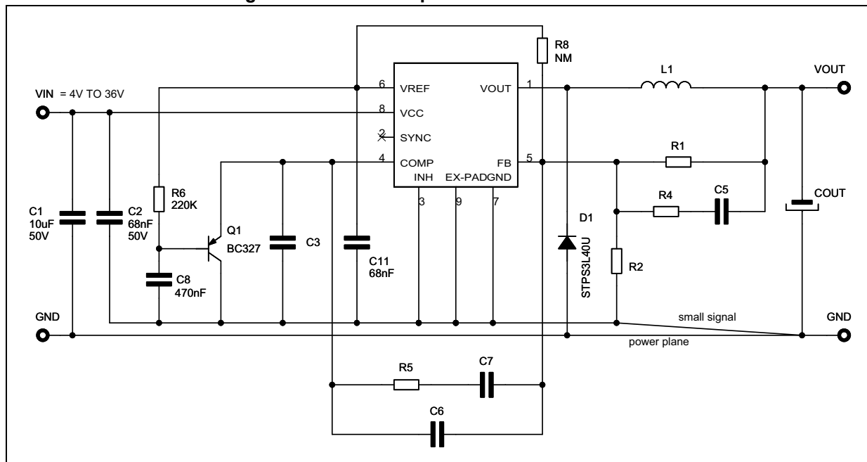
Figure 27. MLCC compensation network circuit
