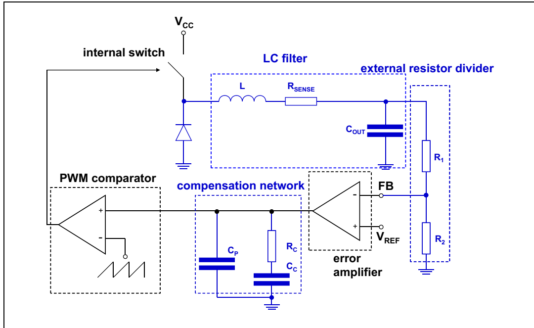
Figure 8. Block diagram of the loop
