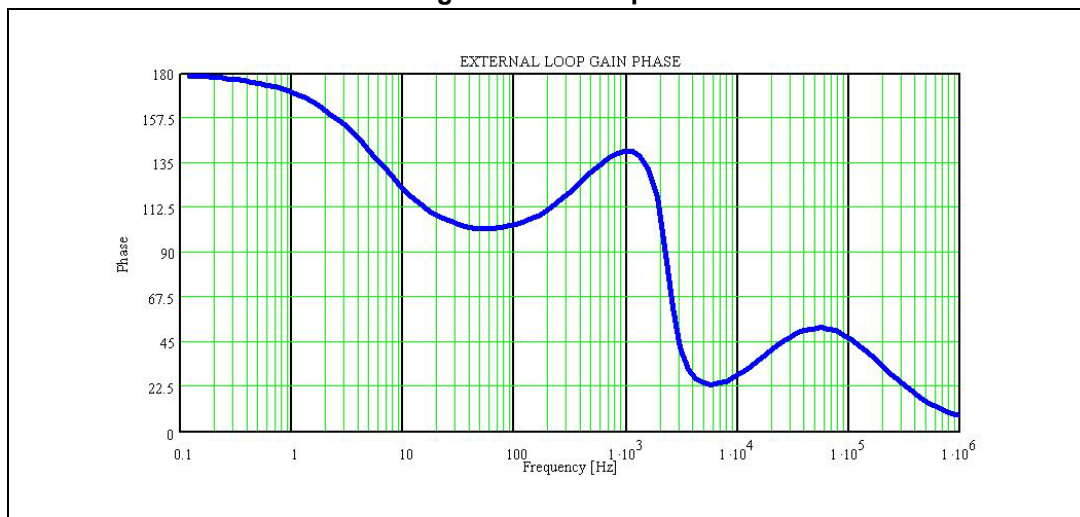
Figure 11. Phase plot
