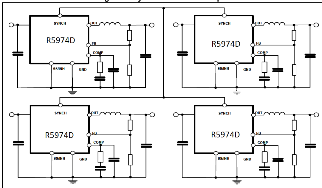
Figure 5. Synchronization example
