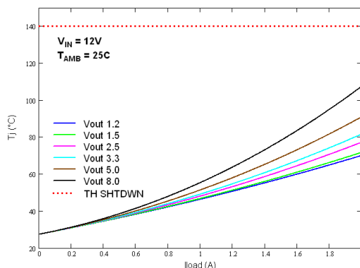
Figure 32. Junction temperature vs. output current ( V_{IN} = 12V )
