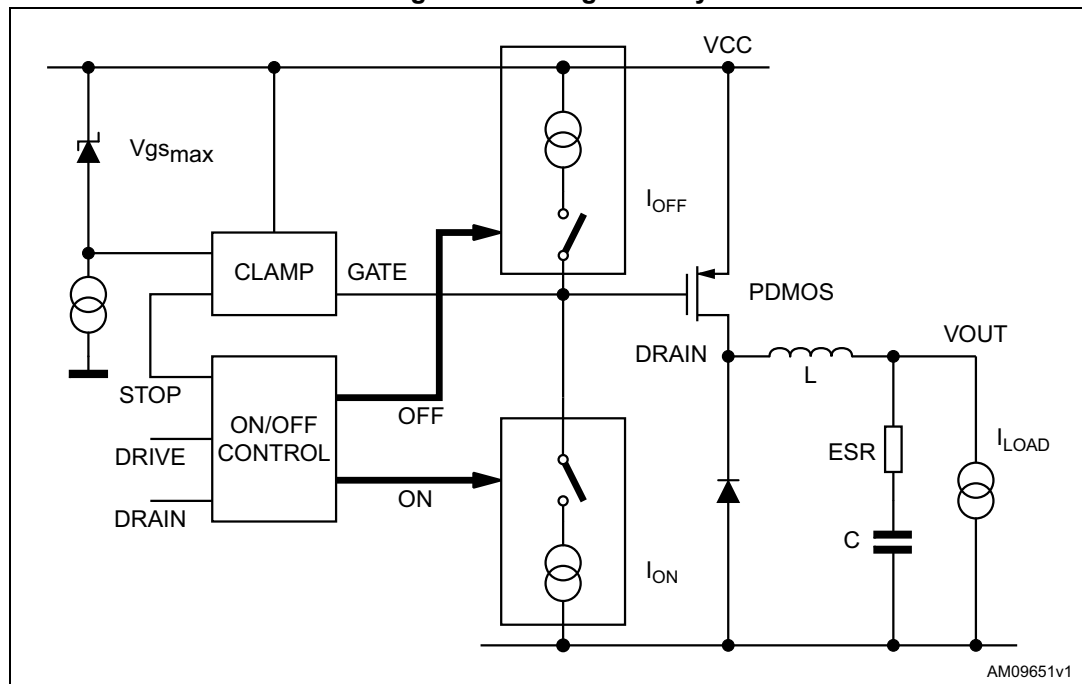
Figure 7. Driving circuitry
