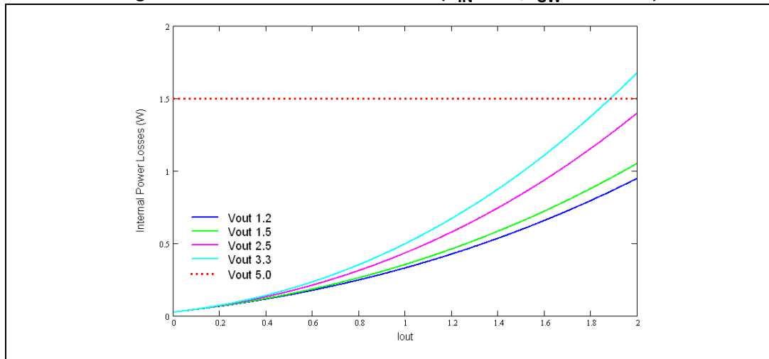
Figure 15. Power losses estimation ( V_{IN} = 5\text{ V} , f_{SW} = 500\text{ kHz} )
