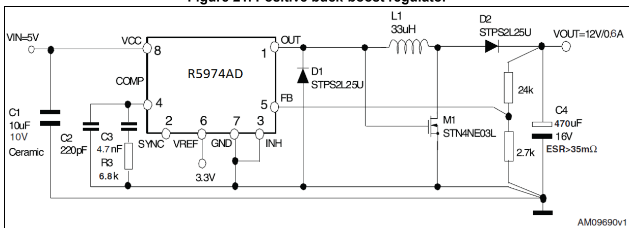
Figure 21. Positive buck-boost regulator
