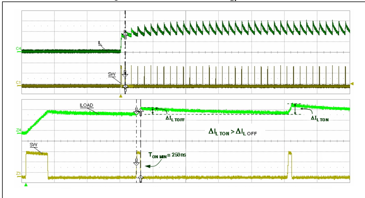
Figure 20. Short-circuit current V_{IN} = 36\text{ V}
