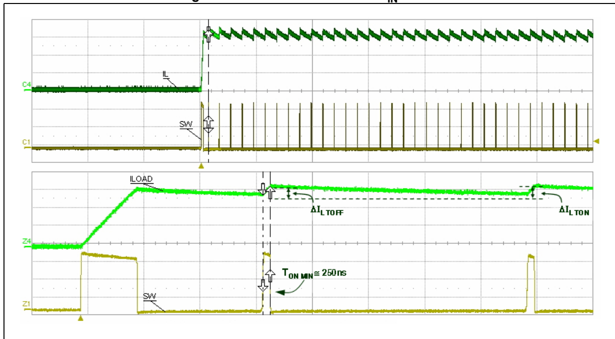
Figure 19. Short-circuit current V_{IN} = 24\text{ V}
