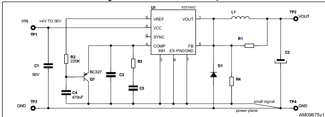
Figure 27. Soft-start network example
