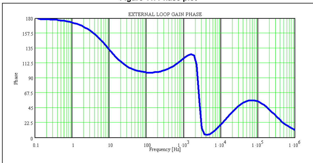
Figure 11. Phase plot
