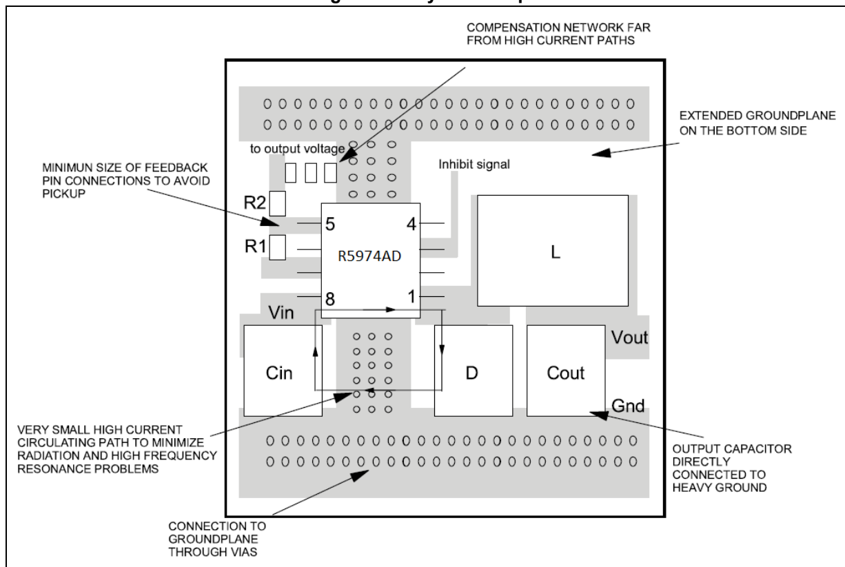
Figure 13. Layout example
