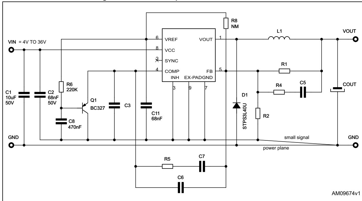
Figure 26. MLCC compensation network circuit
