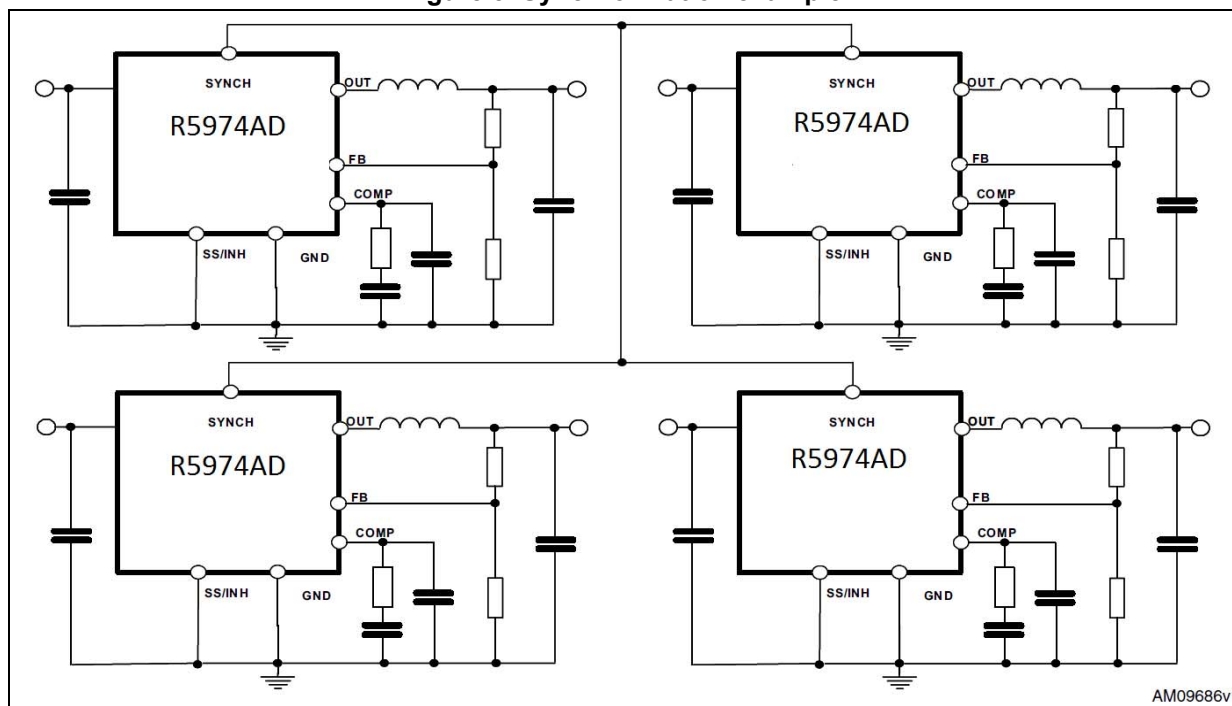
Figure 5. Synchronization example
