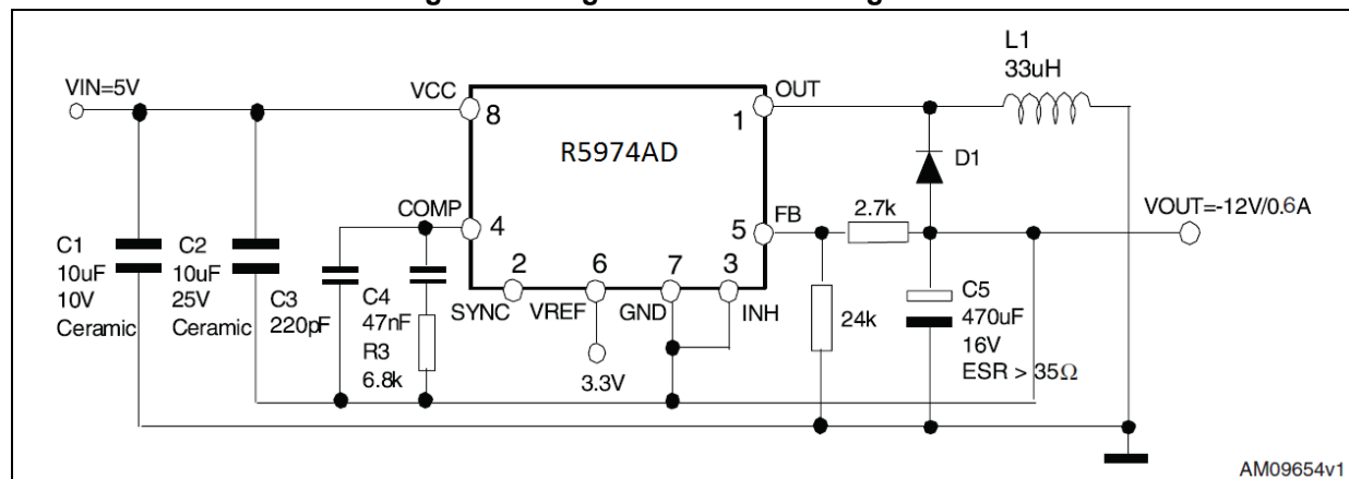
Figure 22. Negative buck-boost regulator
