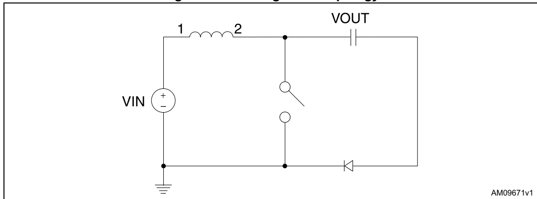
Figure 23. Floating boost topology
