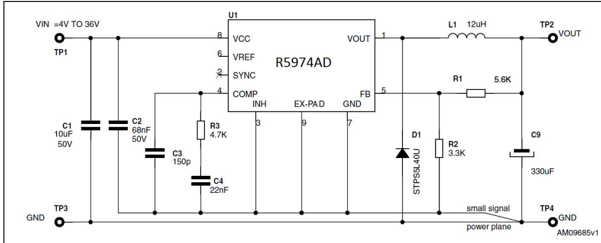
Figure 12. Application schematic
