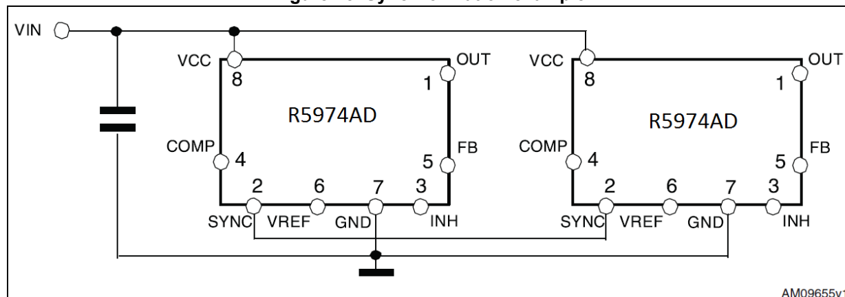
Figure 25. Synchronization example
