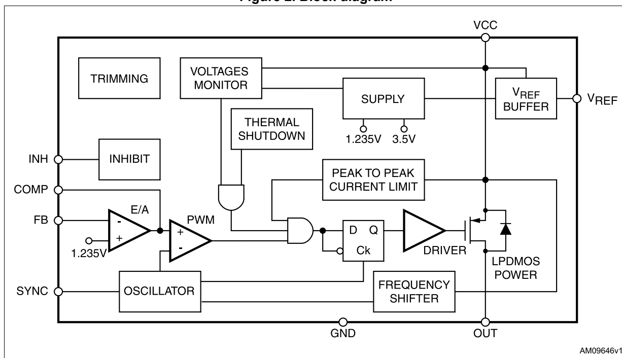
Figure 2. Block diagram
