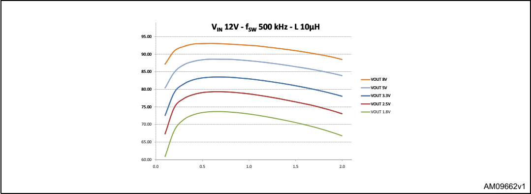
Figure 34. Efficiency vs. output current ( V_{IN} = 12\text{ V} )
